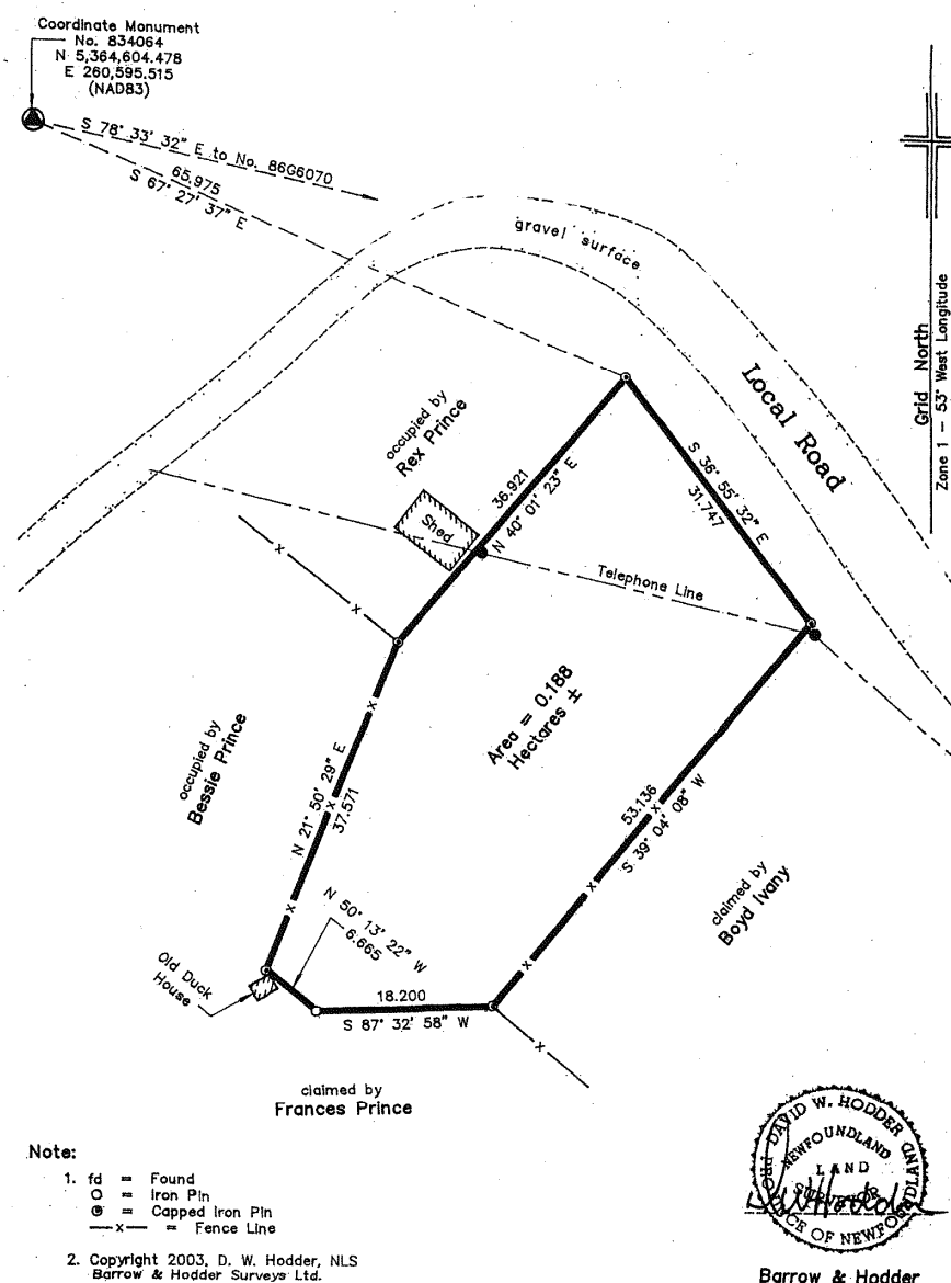
PLAN SHOWING LAND SURVEYED FOR Kay Prince Princeton, NL
