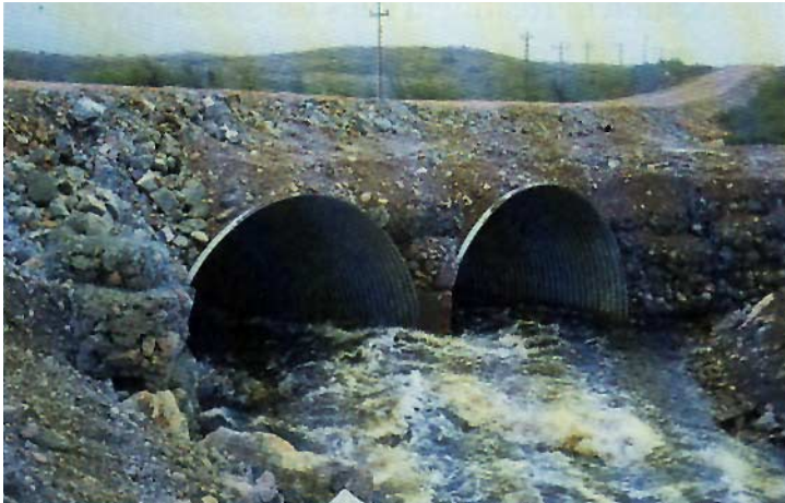
(a) Bottomless arch installation.
