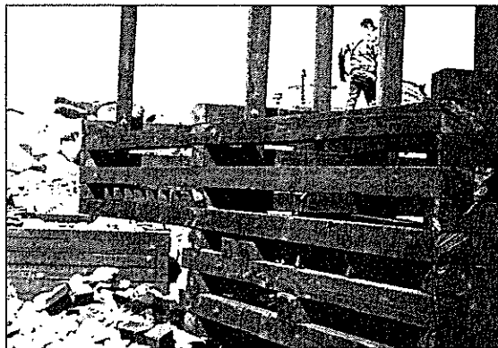
Timber crib construction for marine environment.
