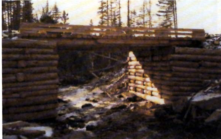
Figure 4.16 Untreated or pressure treated wood should be used for timber crib construction.
