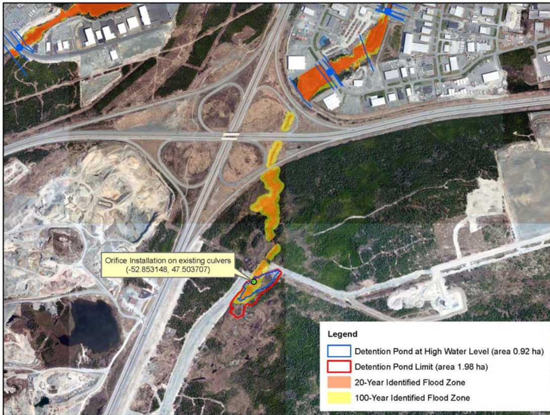
Galway Detention Pond Development
