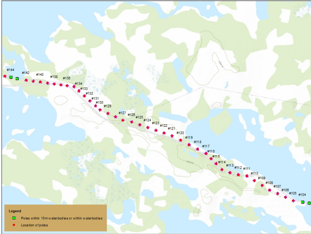
Churchill Falls Gabbro Line Location Map 2
