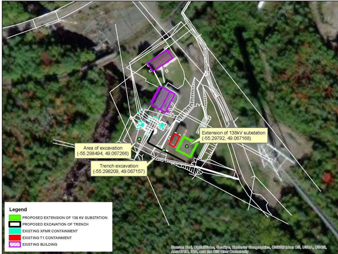
Rattling Brook - Substation Extension and Upgrading of Ground Grid
