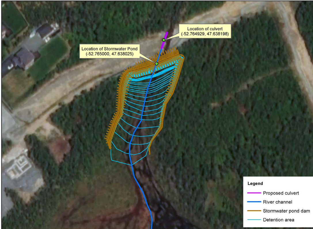
Residential Subdivision development in the Town of Torbay Installation of culvert and construction of stormwater detention pond
