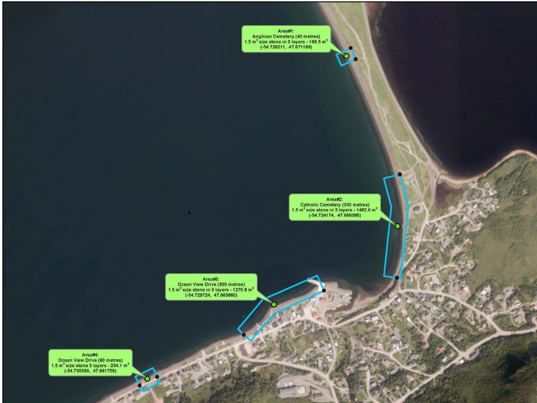
Shoreline Protection Work in the Town of Terrenceville
