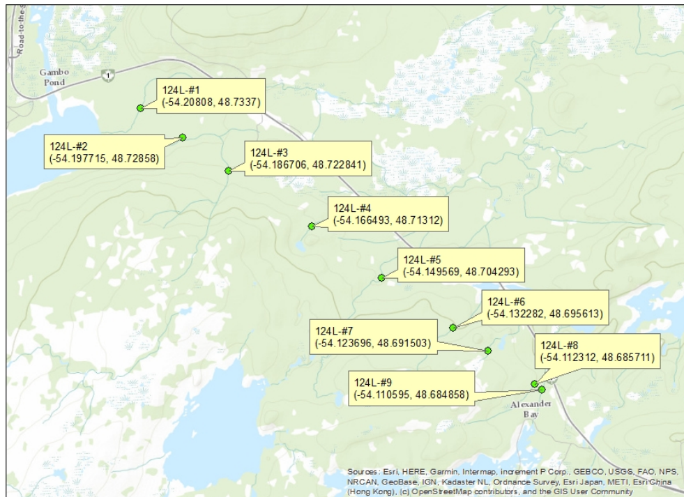
Location of Fordings for 124L - 138 kV Transmission Line Reconstruction
