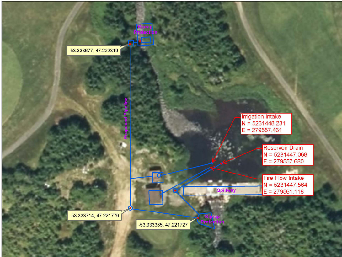
Location Map for Proposed Diversion Pipeline
