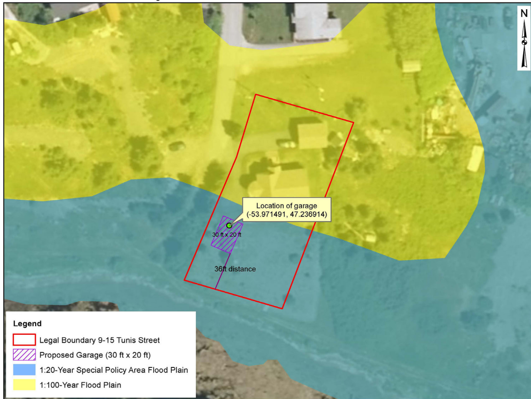
Garage Construction at 9-15 Tunis Street, Placentia
