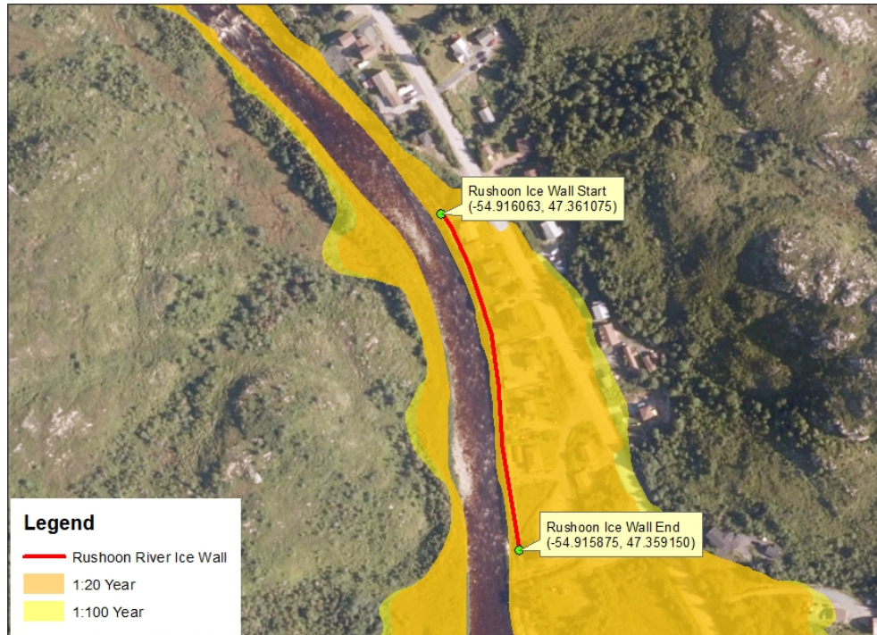
Ice Wall Replacement along Rushoon River, Town of Rushoon
