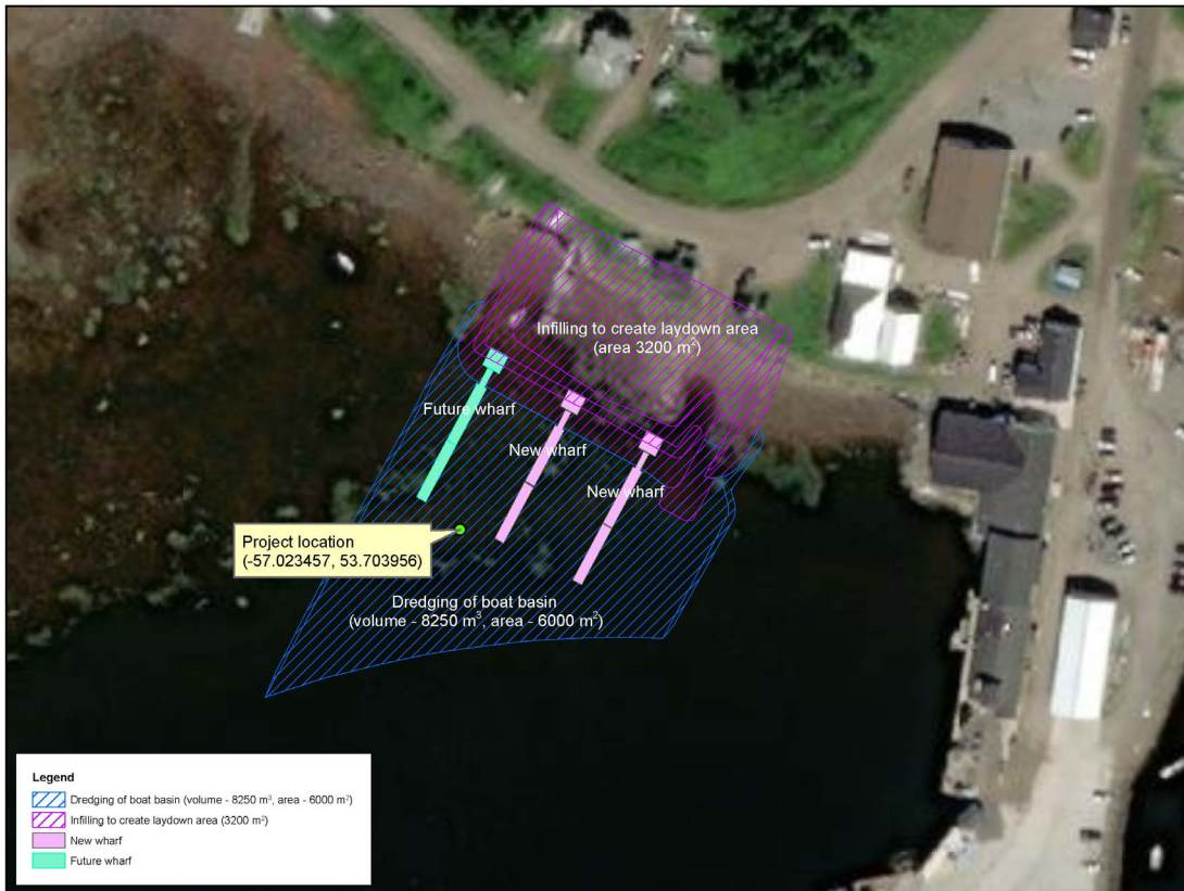
Cartwright Boat Basin Development at Fisheries and Ocean Canada - Small Craft Harbour at Cartwright Harbour
