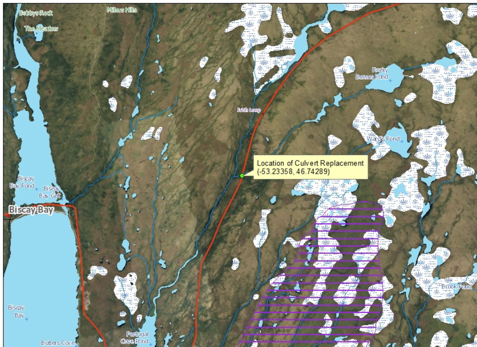
Replace CSP Culvert on Route 10 at km 113.02 South
