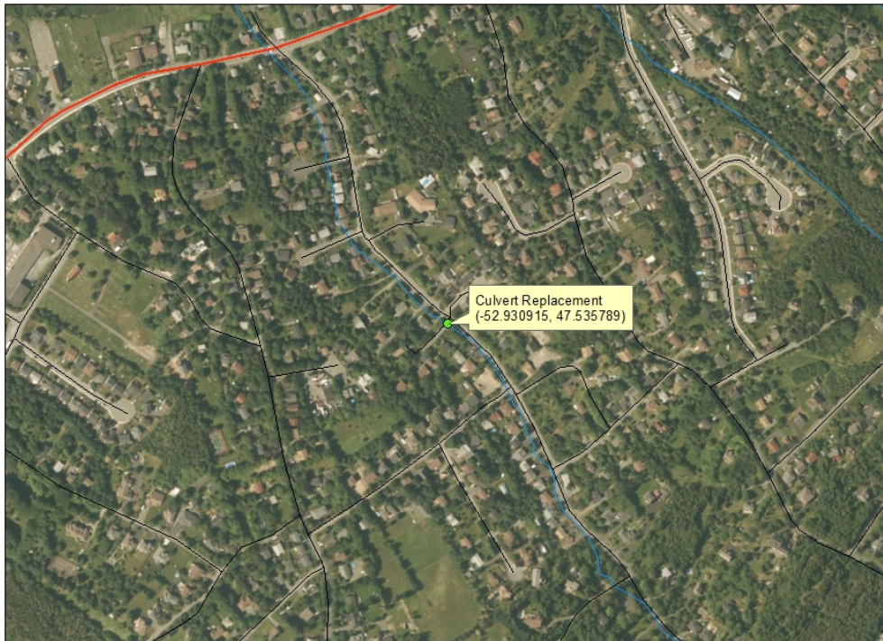
Culvert Replacement along Monument River in the Town of Conception Bay South
