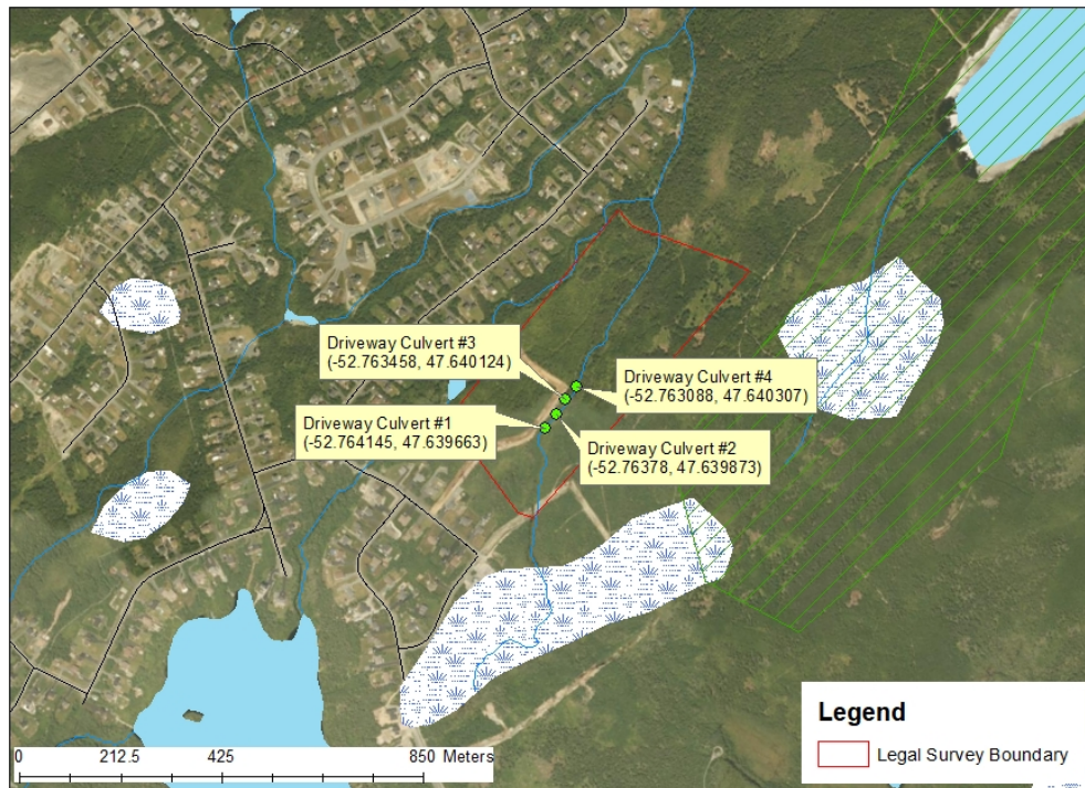
Forest Landing Subdivision Driveway Culverts, Torbay
