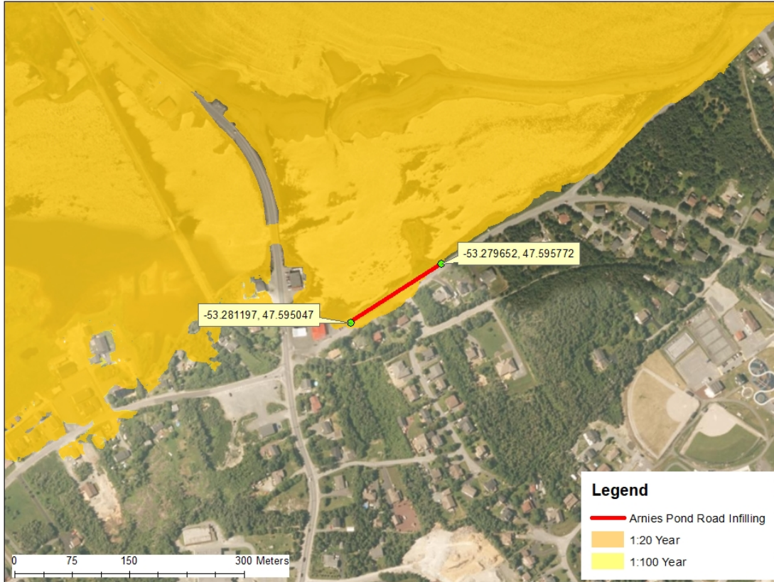
Armour Stone Placement Along Arnies Pond Road, Town of Bay Roberts
