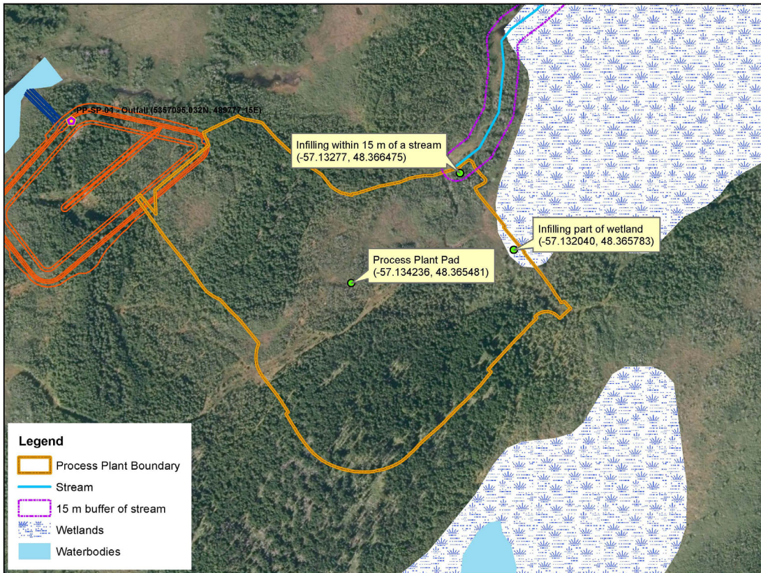
Process Plant Site in Valentine Gold project
