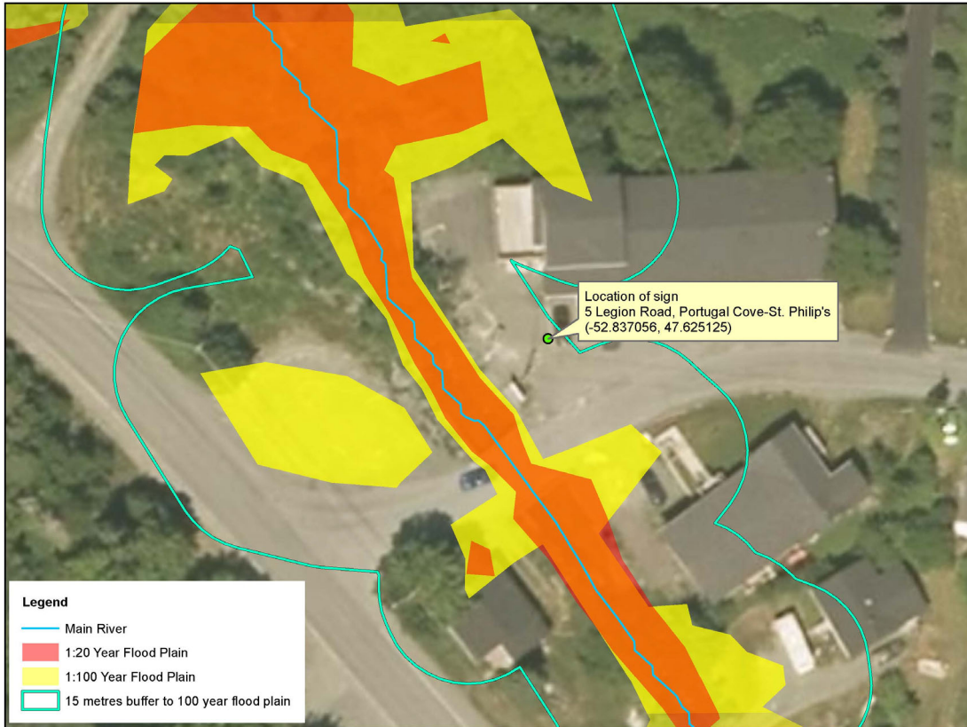
Flood Plain Mapping of Main River at 5 Legion Road, Portugal Cove-St. Philip's
