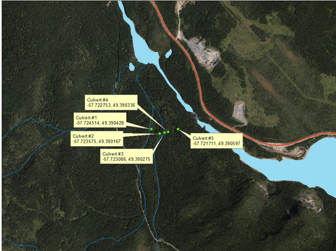
Access Trail Culverts - Lomond River Fishway Enhancement Project
