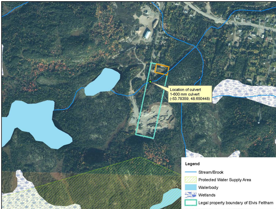
Installation of culvert at 38-40 Tulk's Road, Eastport
