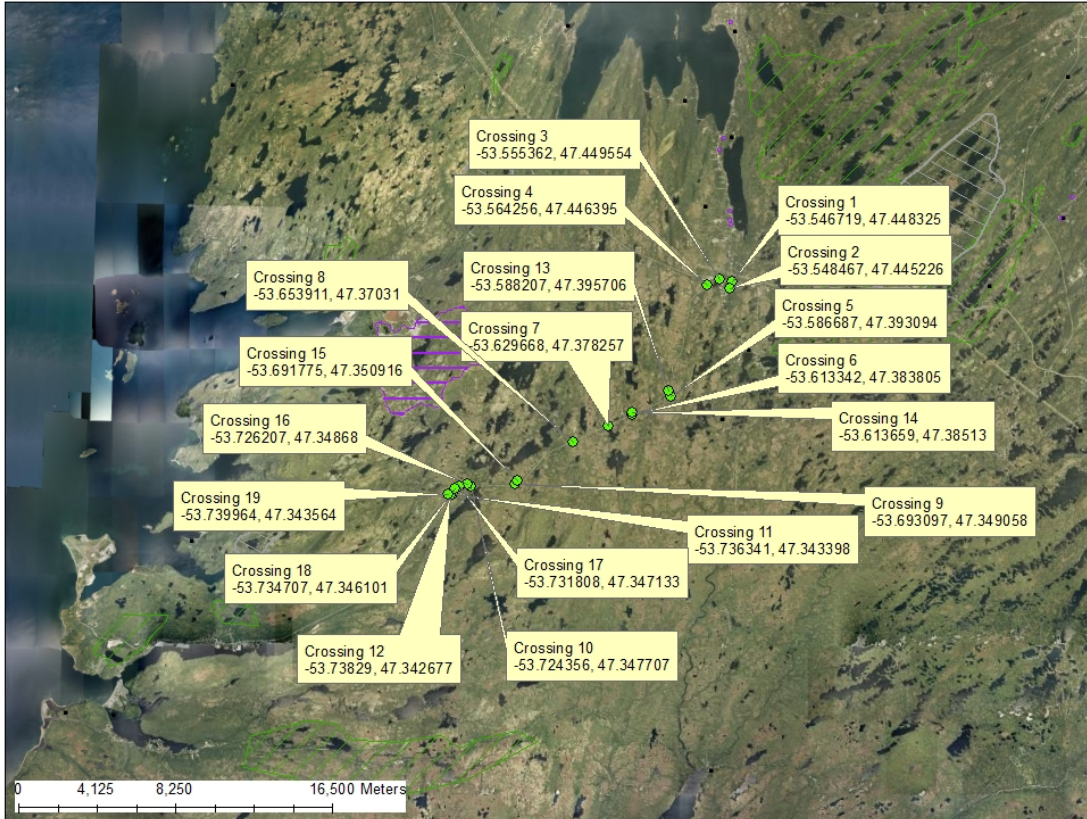
Transmission Line 55L Rebuild - Fording Locations - Northeast of Placentia
