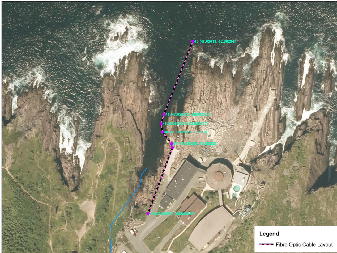
ExxonMobil Canada Fibre Optic Cable at Logy Bay
