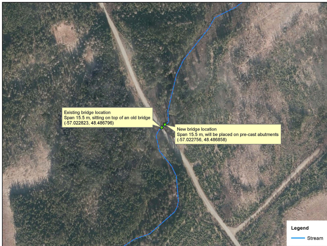
Relocation of bridge in Valentine Gold Project
