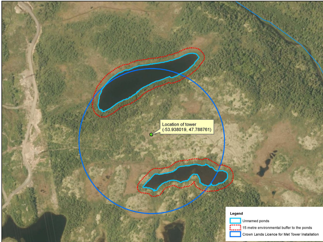
Meteorological Mast Installation for Wind Measurement near Southern Harbour
