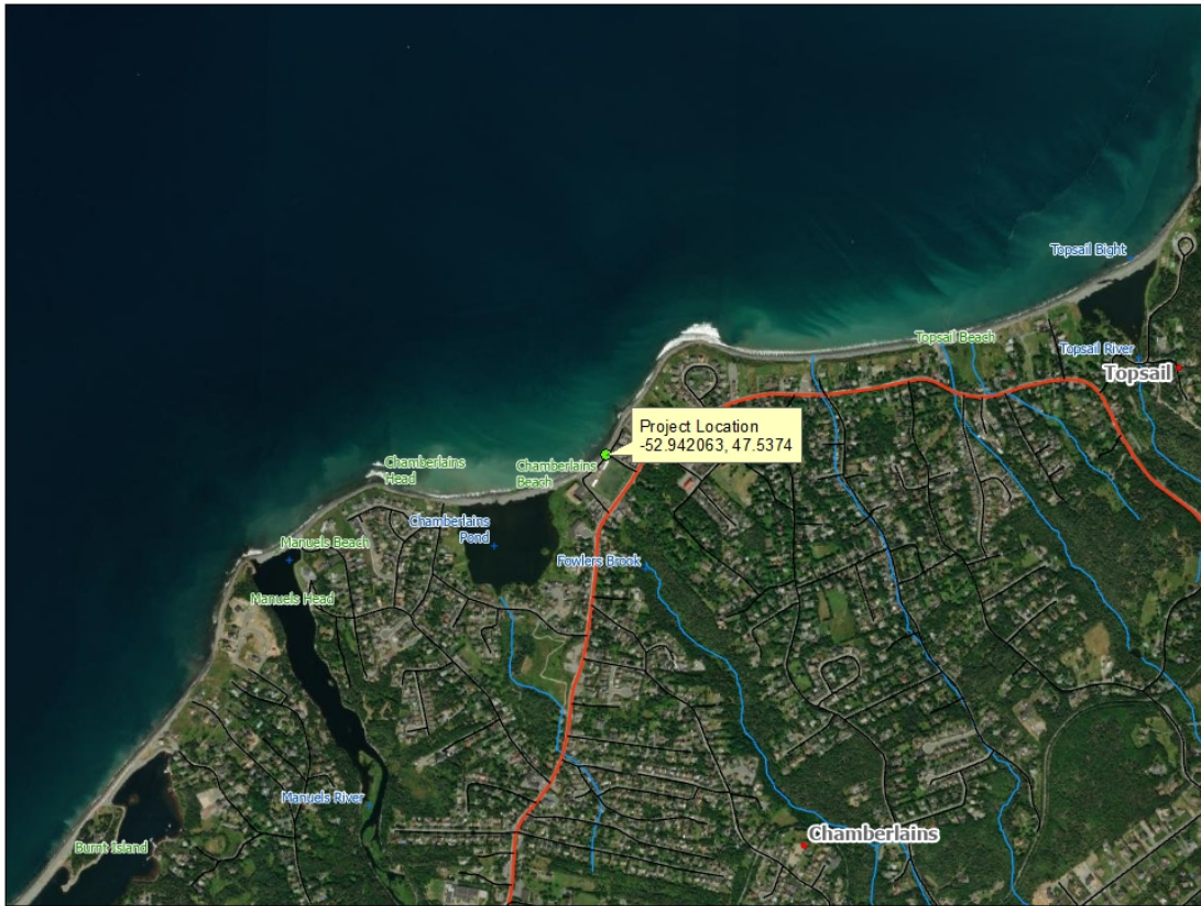
Chamberlains Beach - Existing Culvert Extension and Armourstone Headwall Construction
