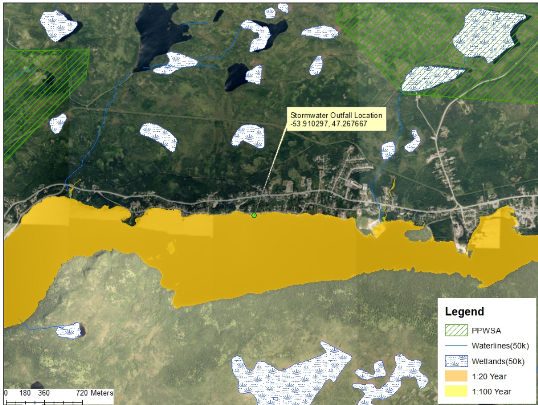
Town of Placentia (Northeast Arm) - Stormwater Outfall in Flood Plain
