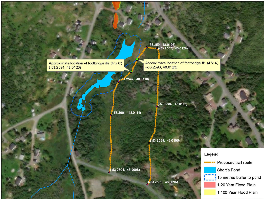
Trail and footbridge construction in Hant's Harbour
