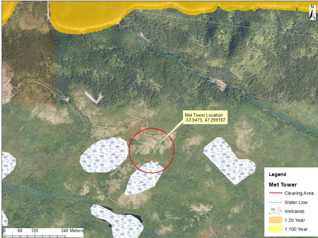
Temporary Meteorological Tower Installation
