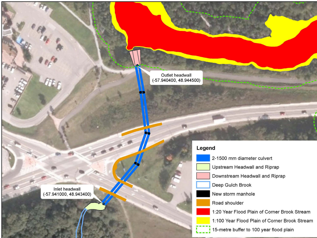
Corner Brook Deep Gulch Culvert Replacement
