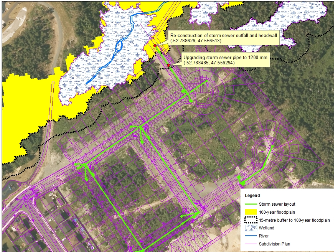
Bristolwood Subdivision Phase 7A, St. John's - Storm Sewer Outfall Upgrading
