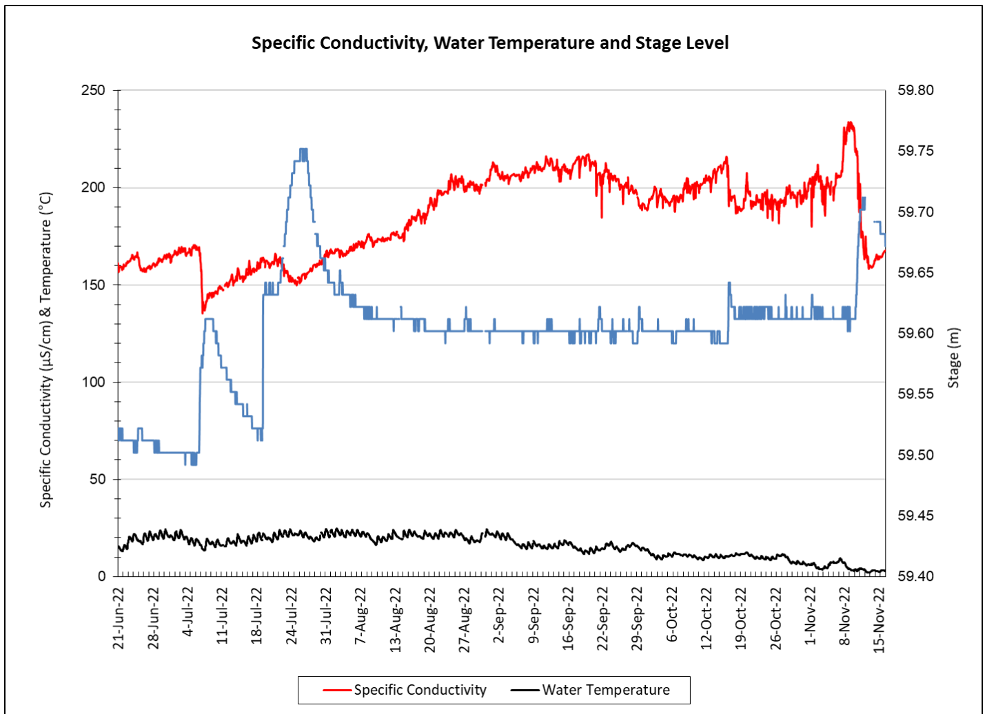
Figure 4: Specific Conductivity and Stage – Outflow of the Steady
