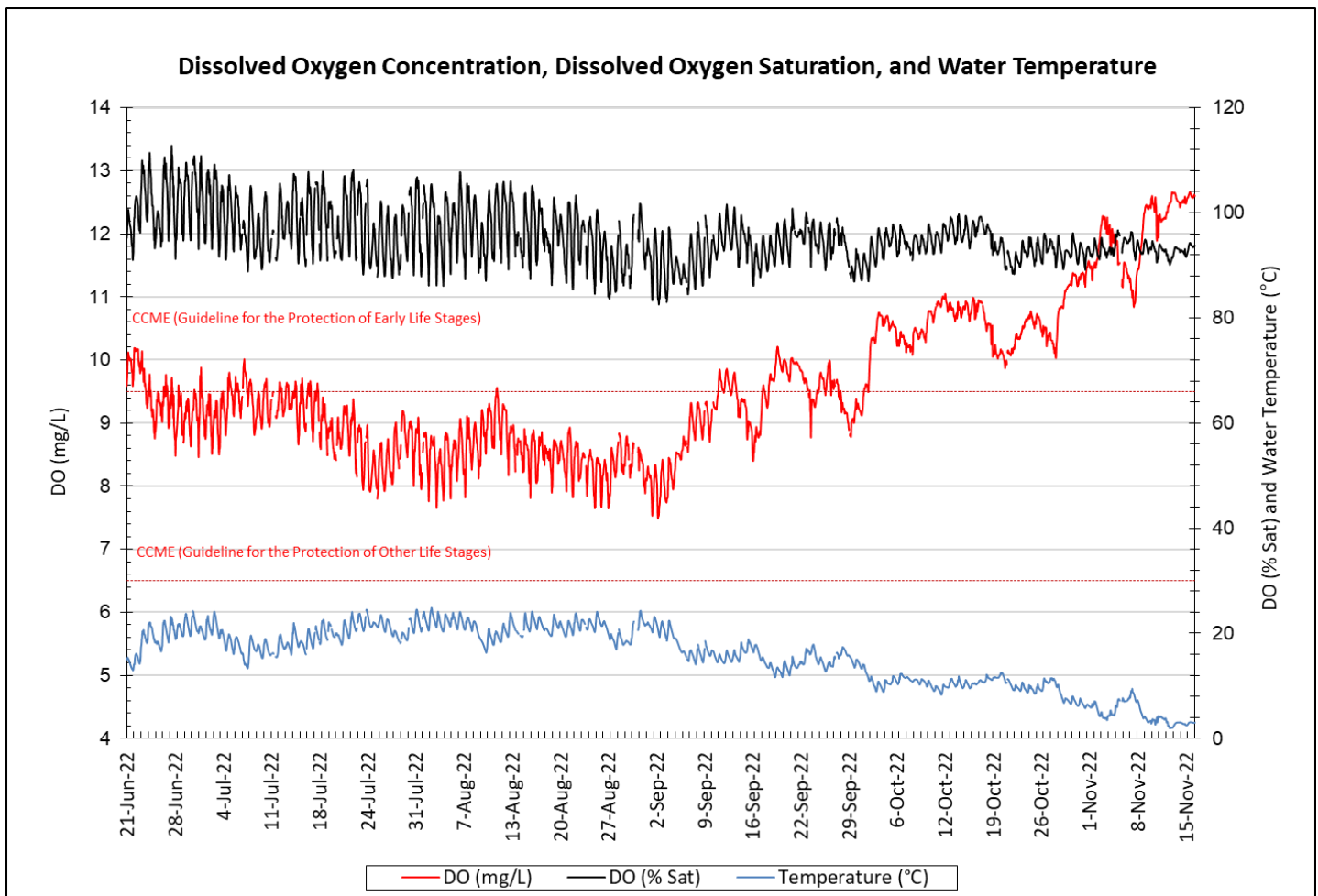
Figure 5: Dissolved Oxygen Concentration, Saturation and Water Temperature – Outflow of the Steady
