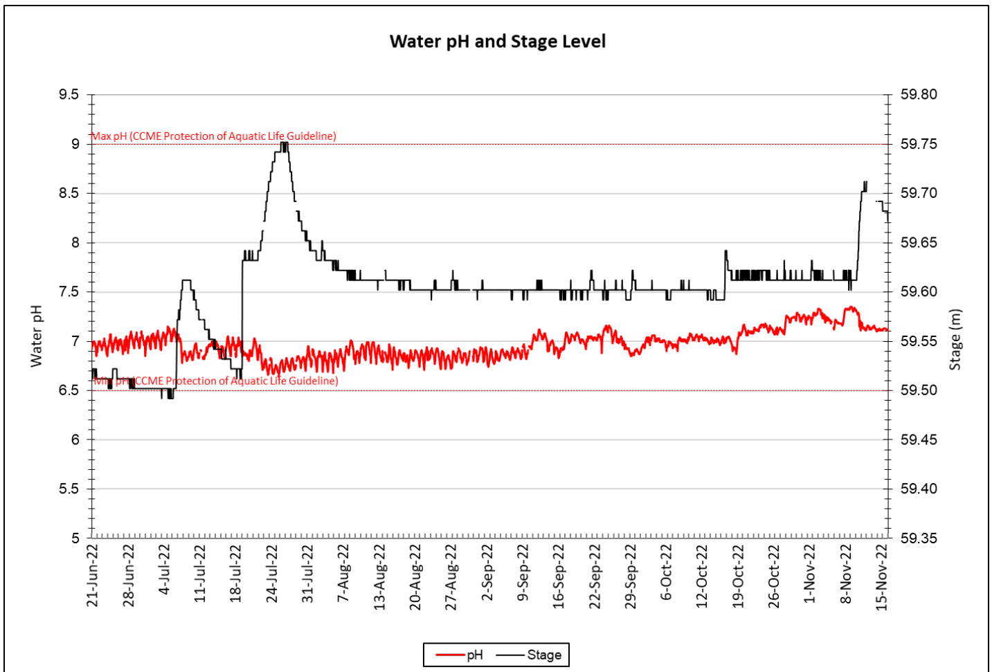
Figure 3: pH and Stage – Outflow of the Steady
