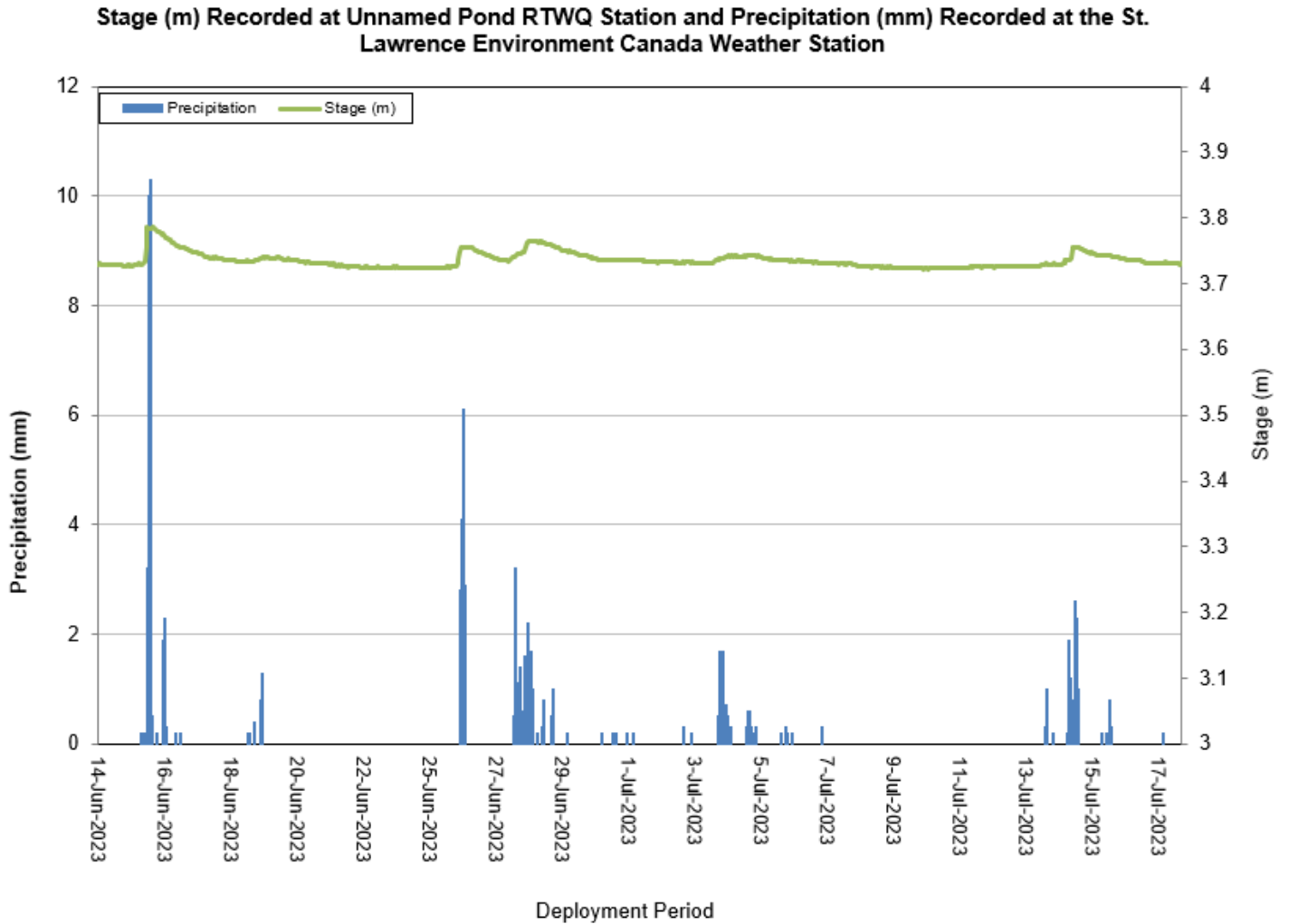
Figure 14: Daily averaged stage values and total precipitation.
