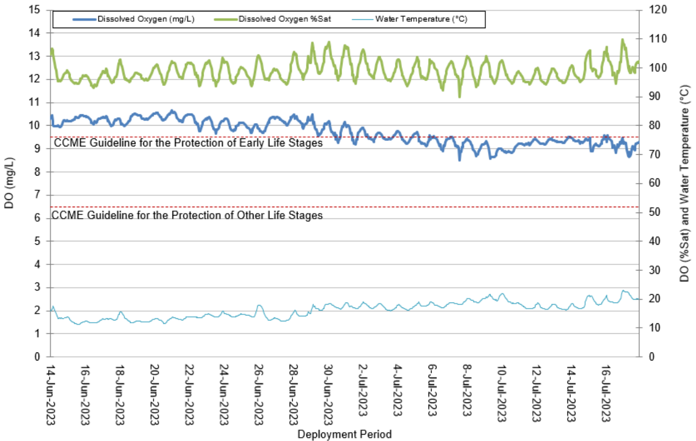
Dissolved Oxygen Concentration (mg/L) and %Sat ) at John Fitzpatrick RTWQ Station
