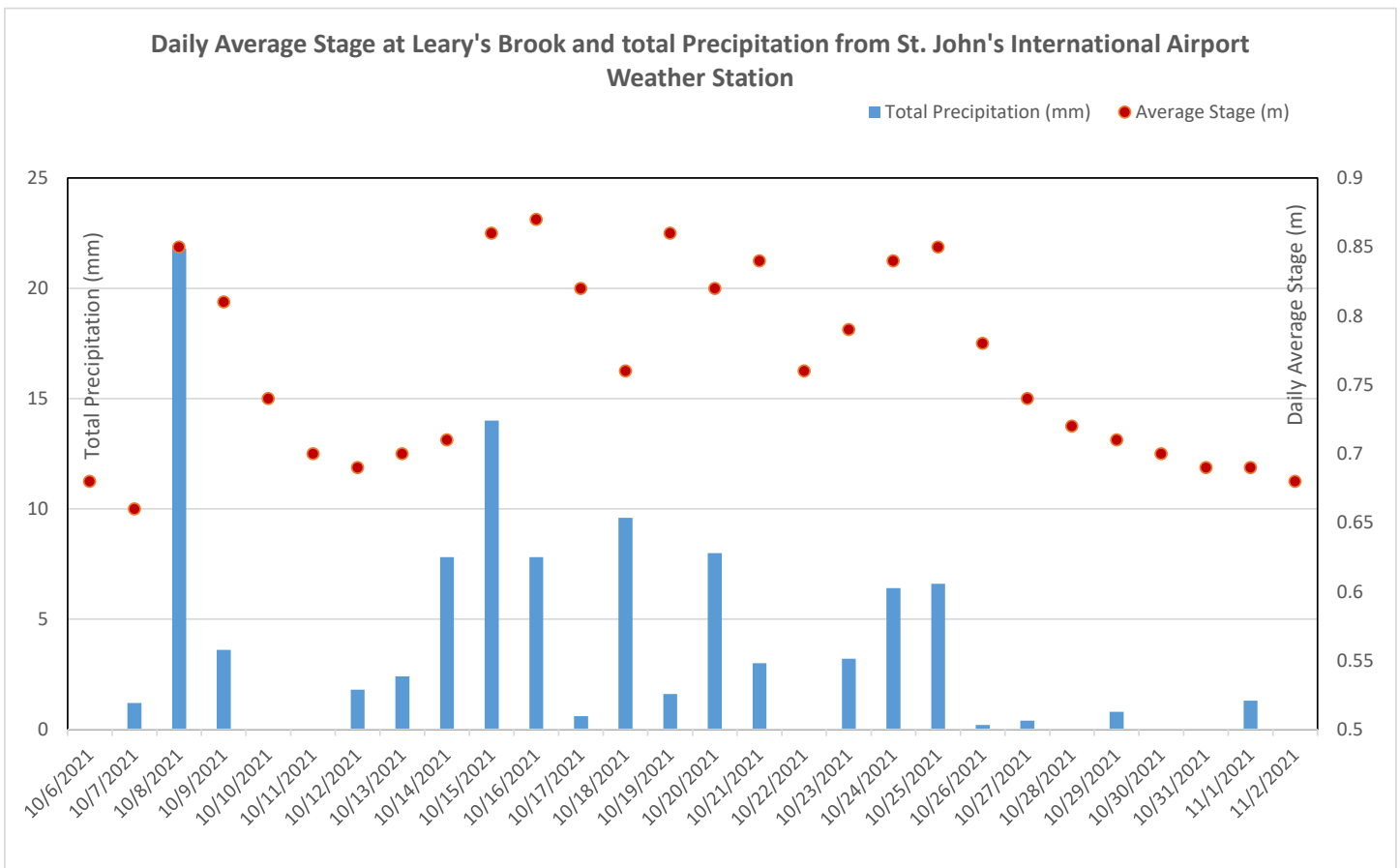
Figure 7: Daily average stage values (m) from Leary's Brook and daily total precipitation values (mm) from St. John's International Airport.
