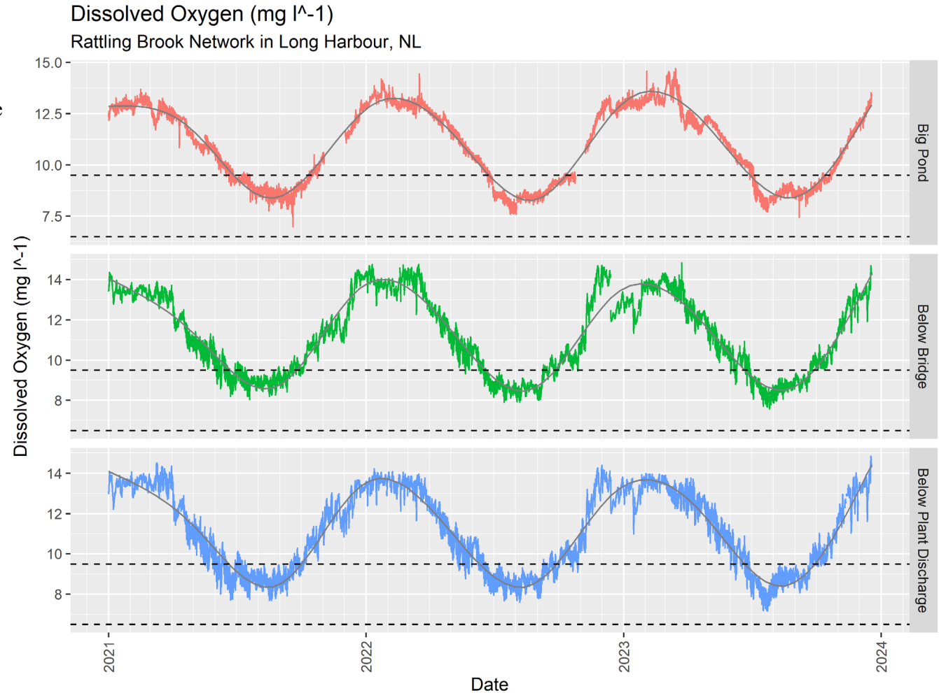
Figure 6: Dissolved oxygen at Rattling Brook from 2021 to 2023
