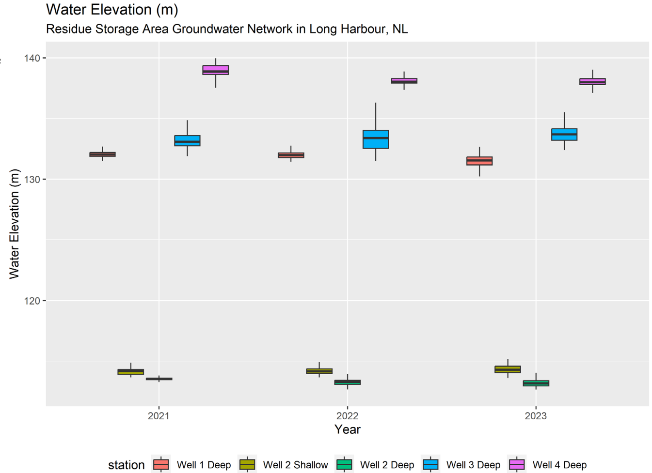
Figure 18: Boxplots of water elevation at the Residue Storage Area from 2021 to 2023
