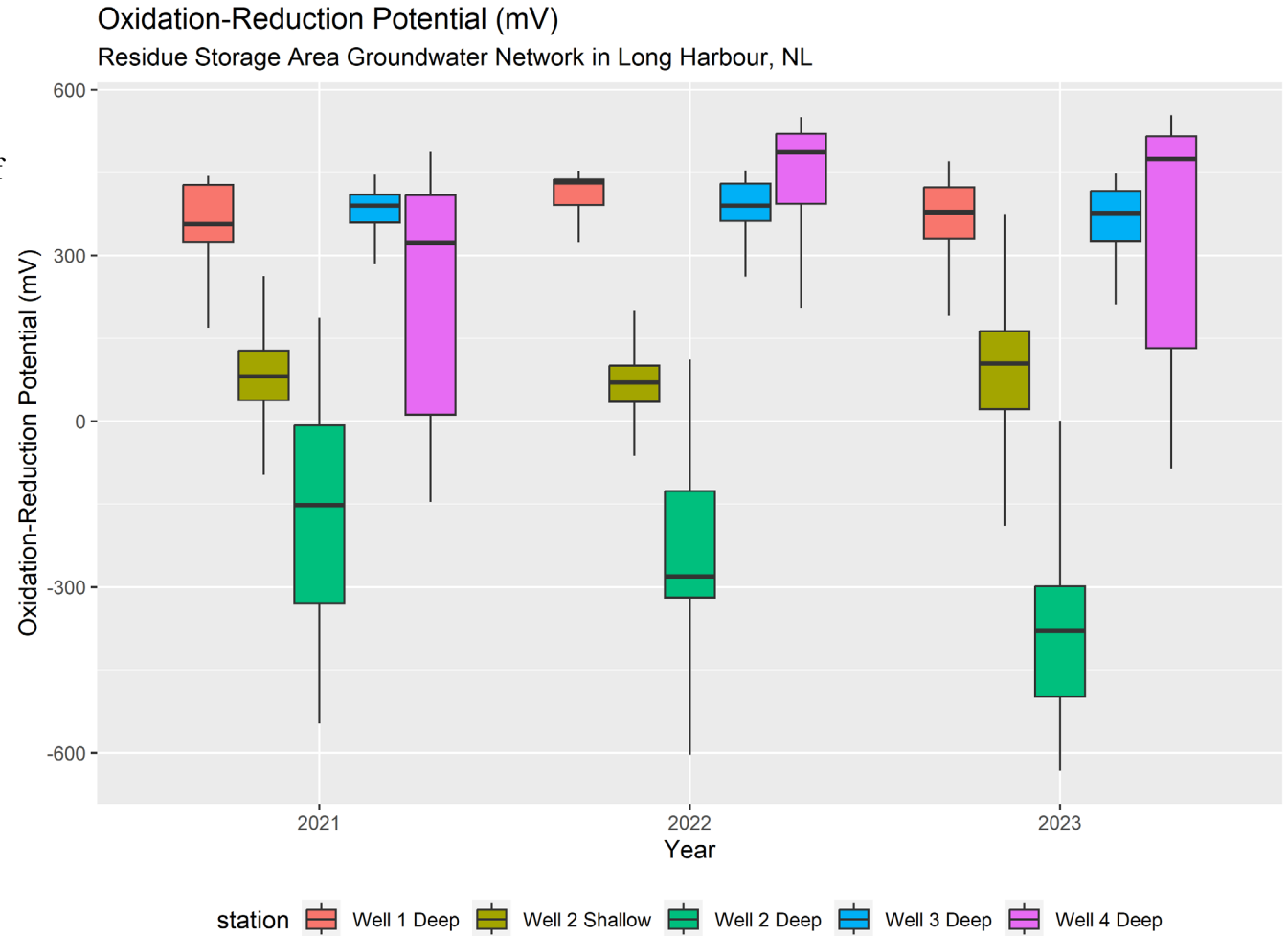
Figure 16: Boxplots of Oxidation-Reduction Potential at the Residue Storage Area from 2021 to 2023
