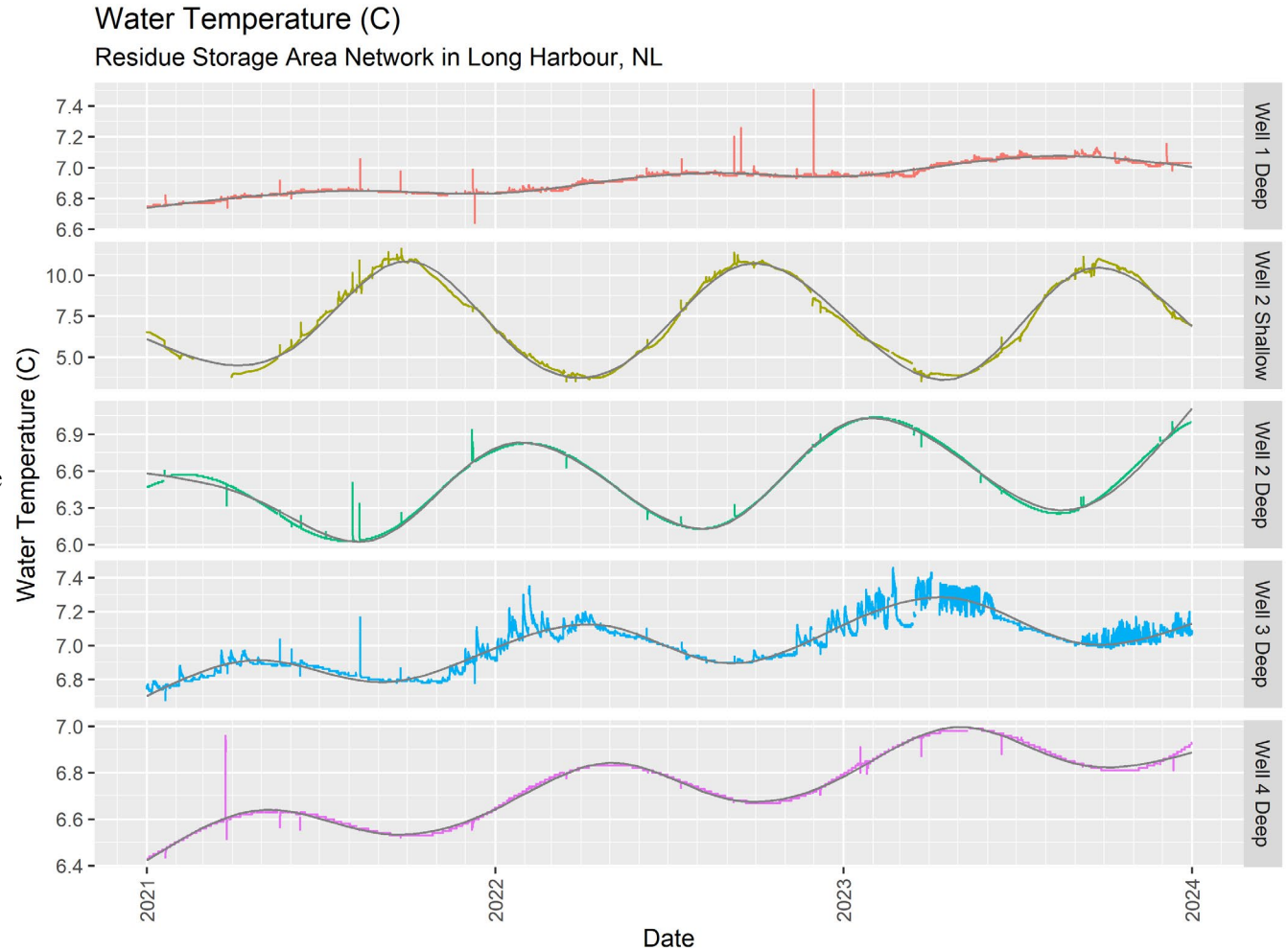
Figure 9: Water temperature at the Residue Storage Area from 2021 to 2023
