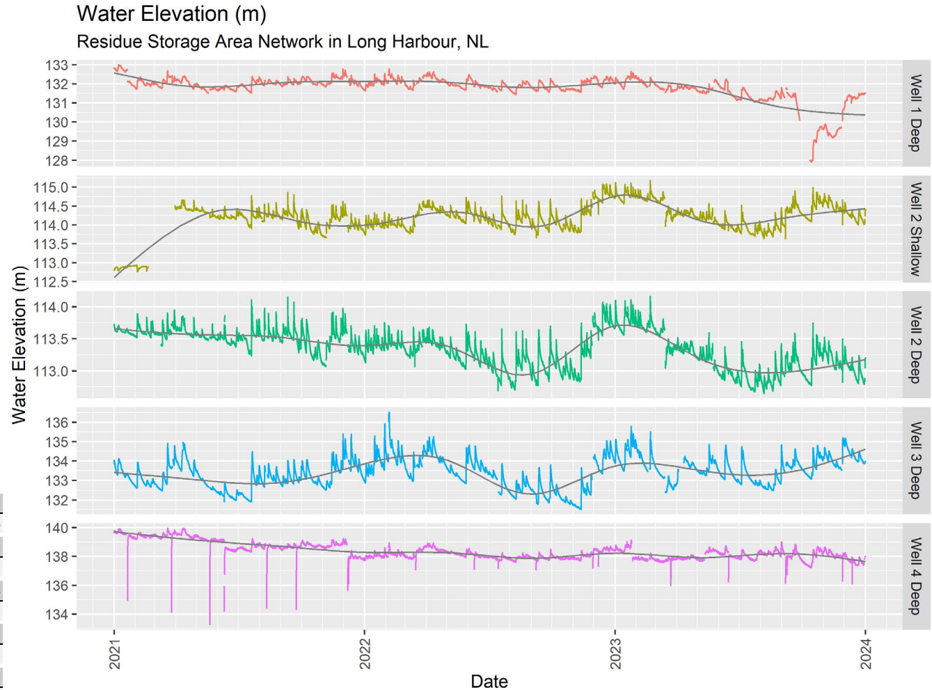
Figure 17: Water elevation at the Residue Storage Area from 2021 to 2023
