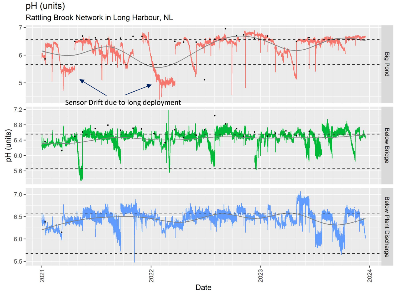
Figure 4: pH at Rattling Brook from 2021 to 2023
