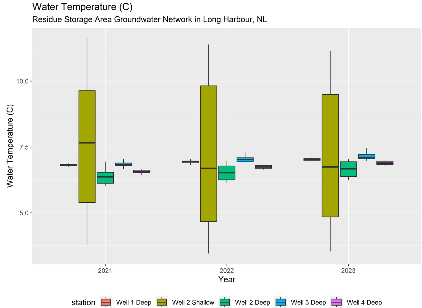
Figure 10: Boxplots of water temperature at the Residue Storage Area from 2021 to 2023
