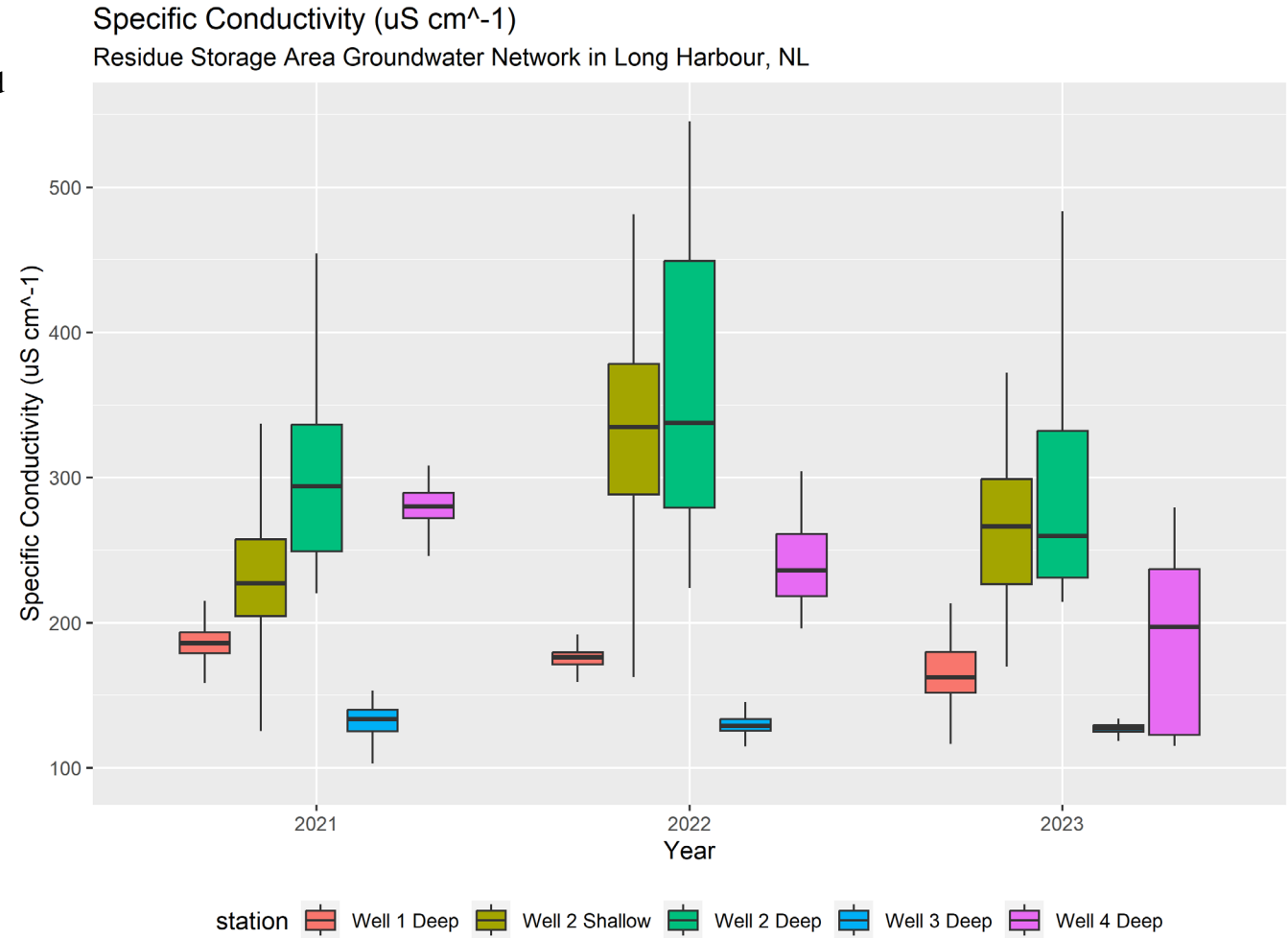
Figure 14: Boxplots of specific conductivity at the Residue Storage Area from 2021 to 2023
