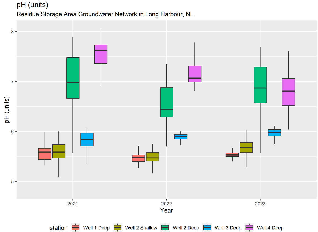
Figure 12: Boxplots of pH at the Residue Storage Area from 2021 to 2023
