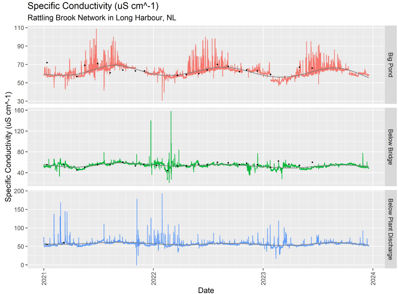
Figure 5: Specific Conductivity at Rattling Brook from 2021 to 2023
