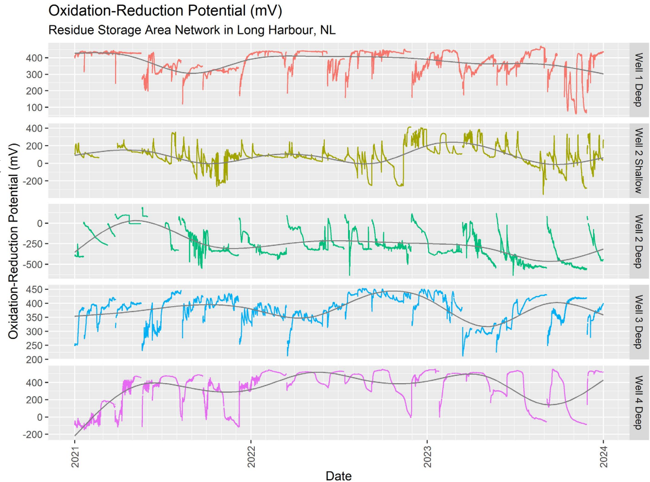
Figure 15: Oxidation-Reduction Potential at the Residue Storage Area from 2021 to 2023
