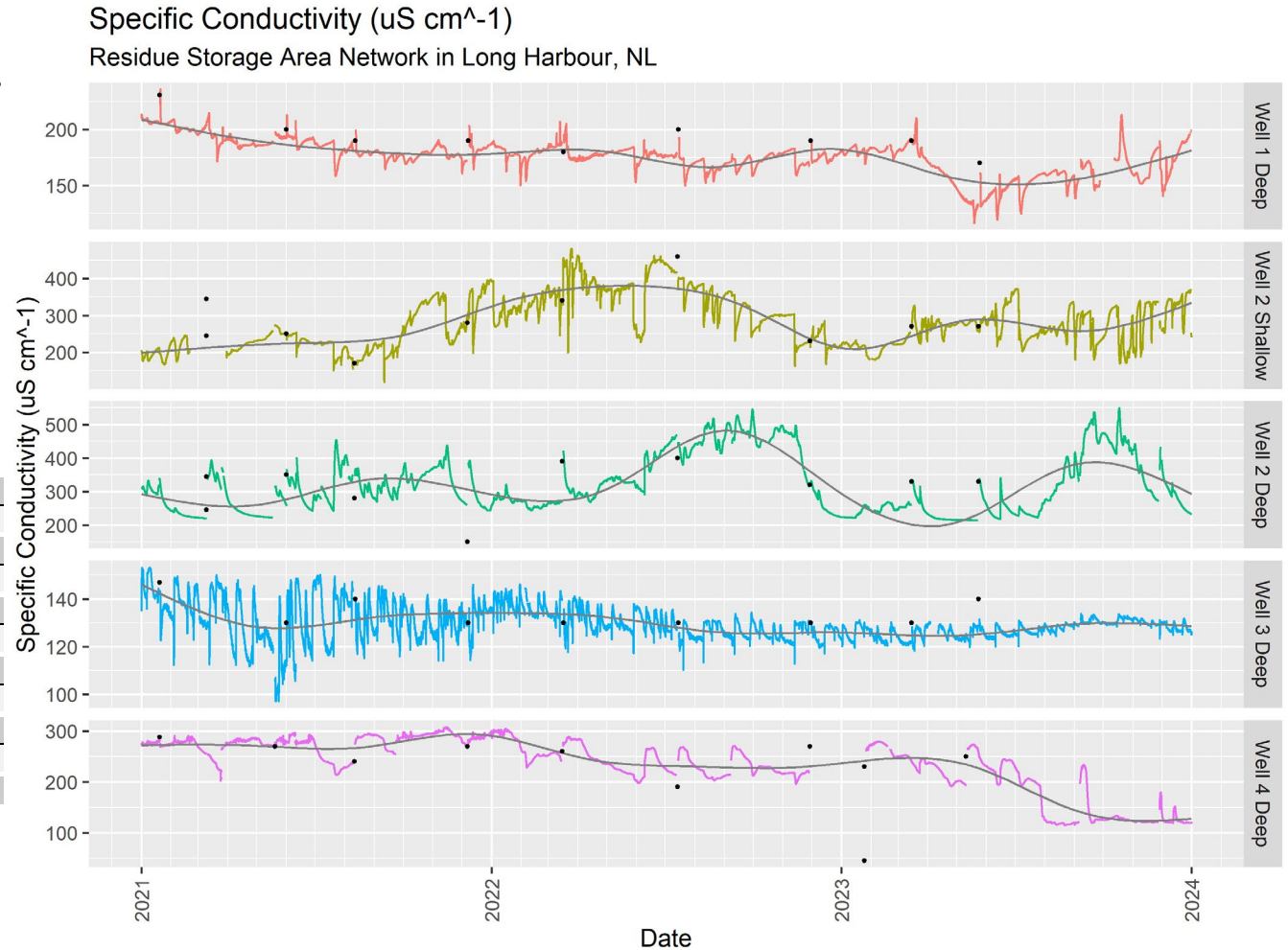
Figure 13: Specific conductivity at the Residue Storage Area from 2021 to 2023
