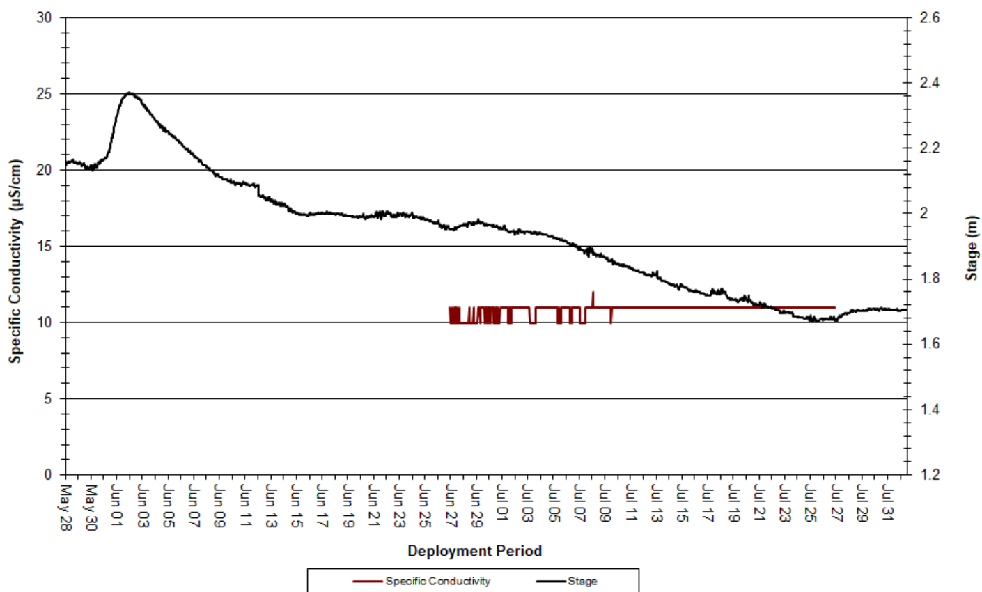
Figure 4: Specific Conductivity & Stage at Reid Brook at Outlet of Reid Pond
