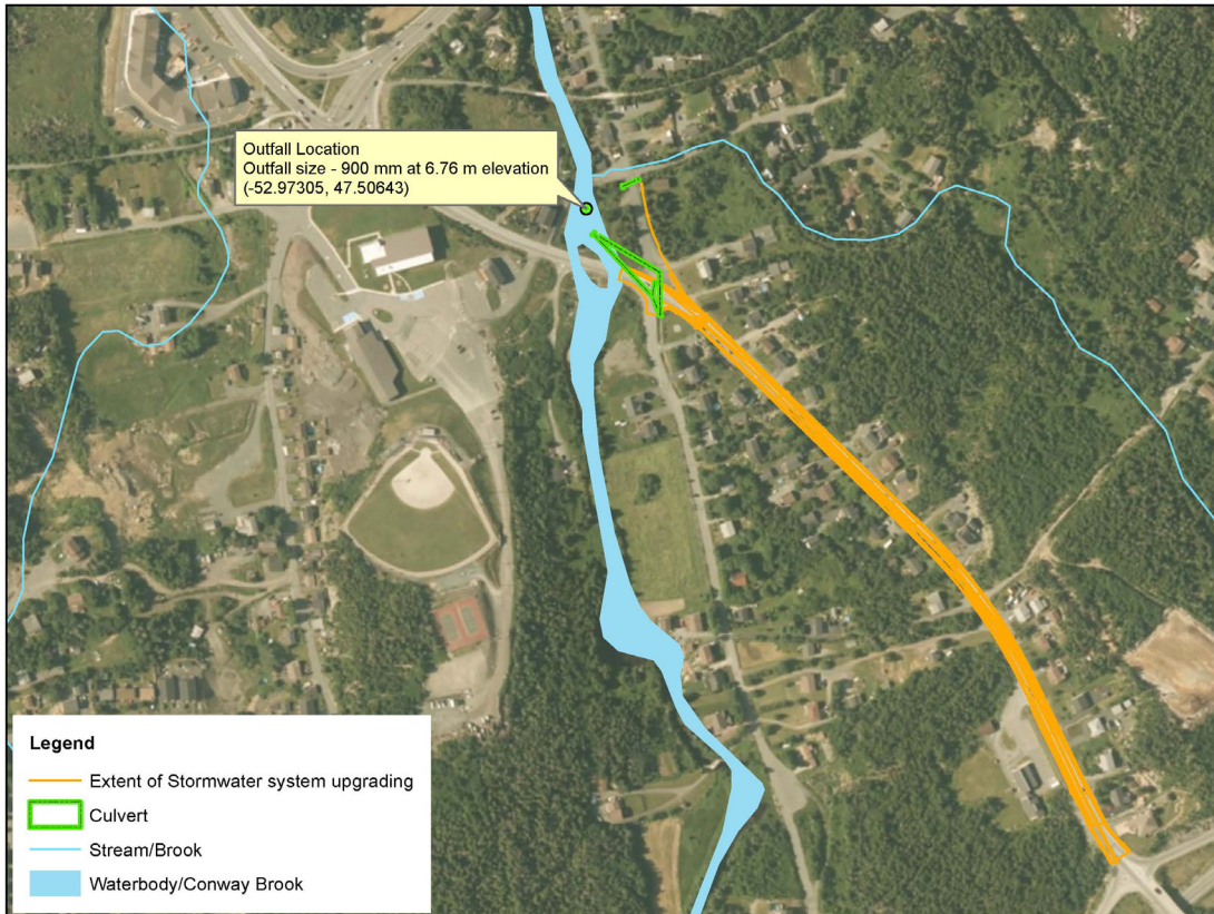
Upgrading of Stormwater System on Minerals Road in Conception Bay South
