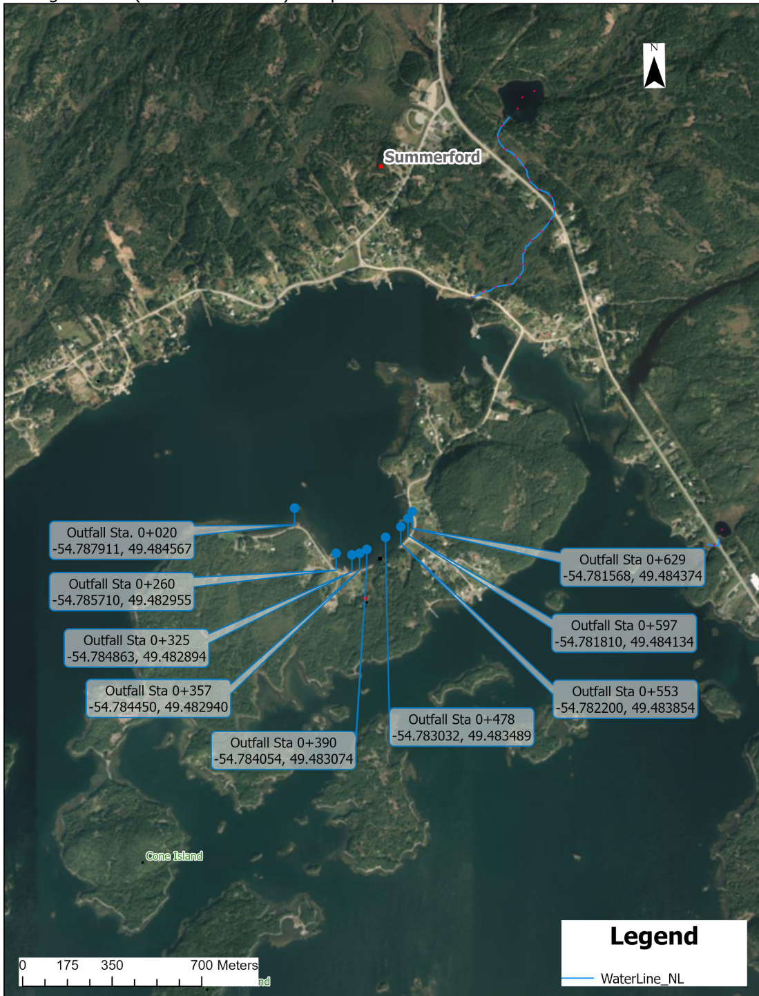
Strong's Island (Summerford Arm) - Replacement of Nine Deteriorated Stormwater Outfalls
