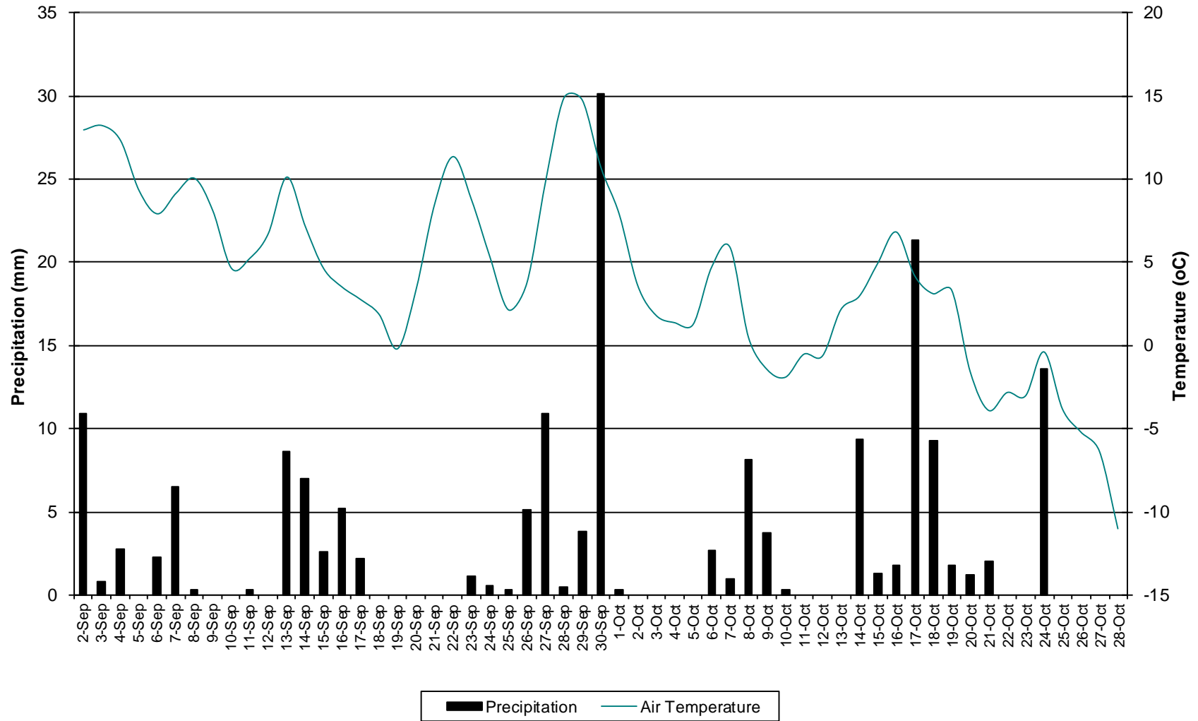
Average Air Temperature and Daily Precipitation: Moosehead Lake, NL September 2 to October 28, 2020
