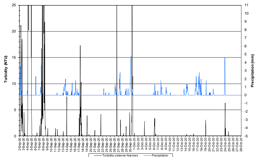
Figure 6b: Turbidity < 25 NTU and Precipitation – Julienne Narrows
