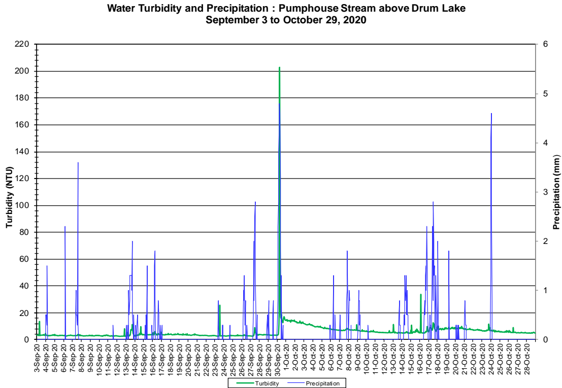
Figure 19a: Turbidity and Precipitation – Pumphouse Stream (Weather data collected from climate station near Moosehead Lake)
