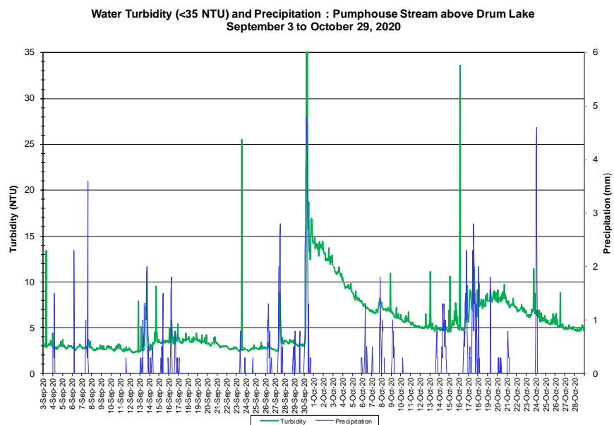
Figure 19b: Turbidity (<35 NTU) and Precipitation – Pumphouse Stream (Weather data collected from climate station near Moosehead Lake)
