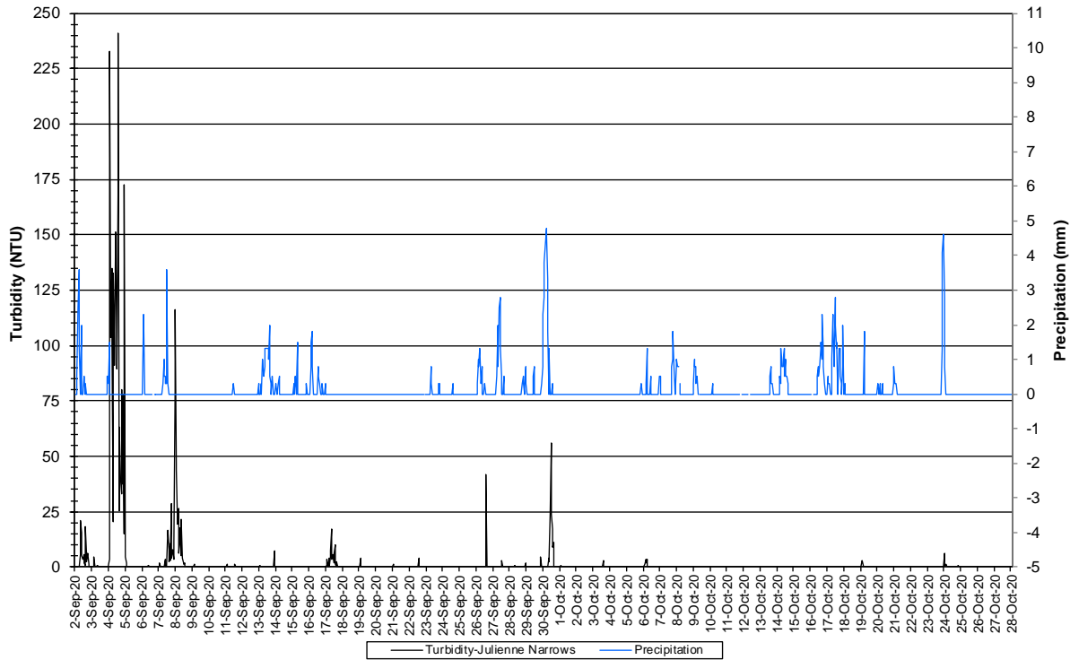
Figure 6a: Turbidity and Precipitation – Julienne Narrows (Weather data collected from climate station near Moosehead Lake)
