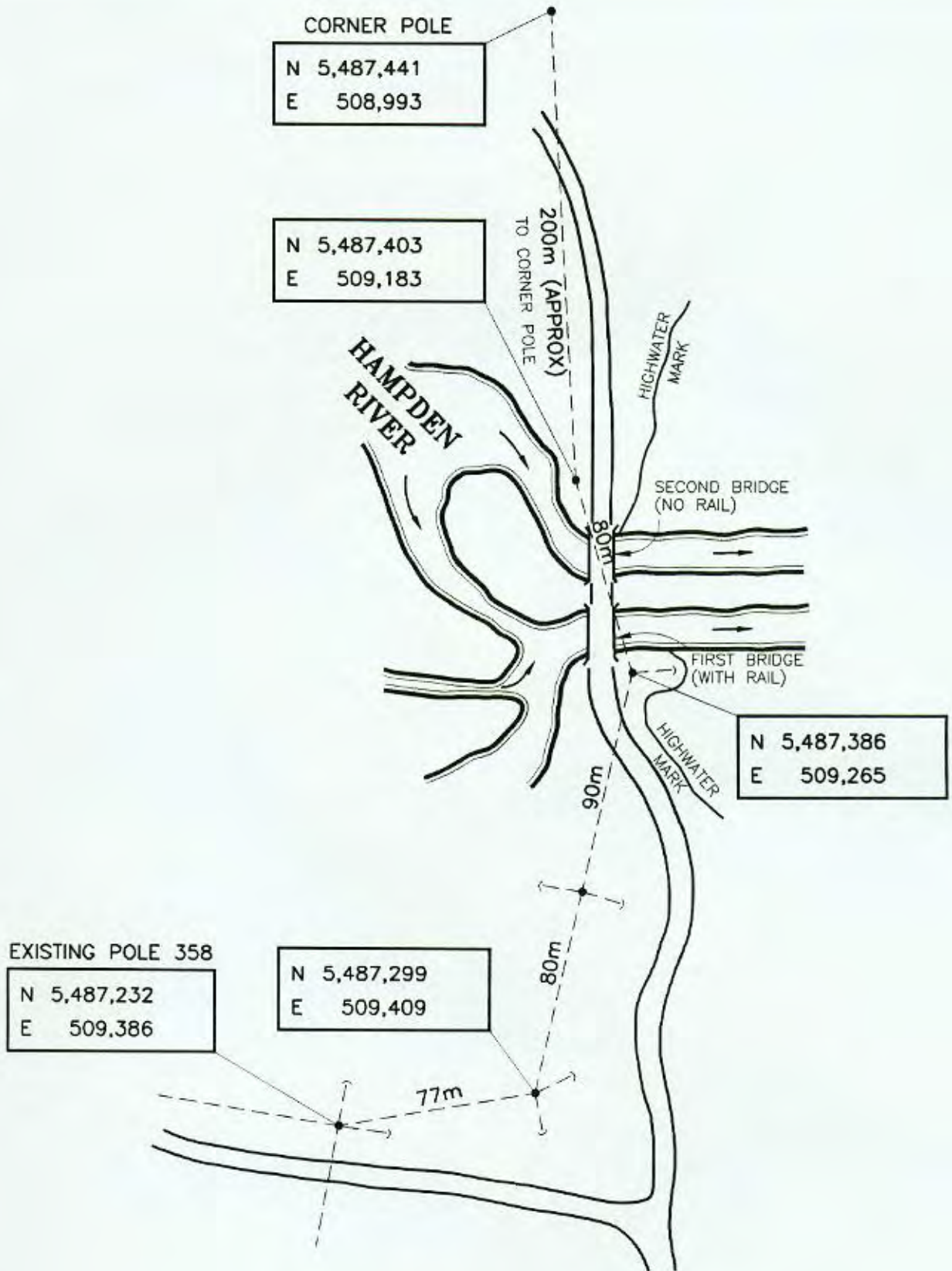
HAMPDEN RIVER CROSSING DETAIL 1 N.T.S.
