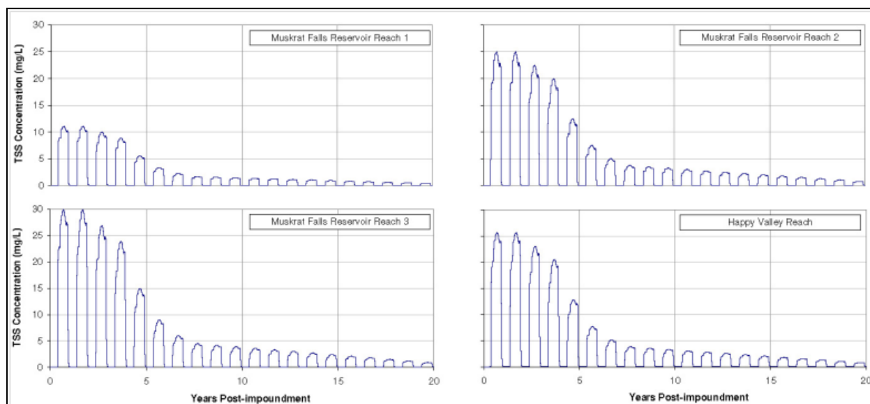
Figure 7.11. Modeled TSS within the Muskrat Reservoir and downstream of Muskrat Falls
