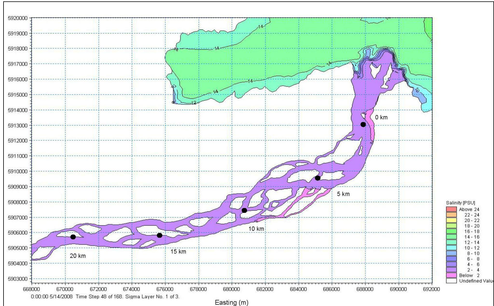
Figure 7.15. Modeled salinities with 30% MAF compensation flow during reservoir filling
