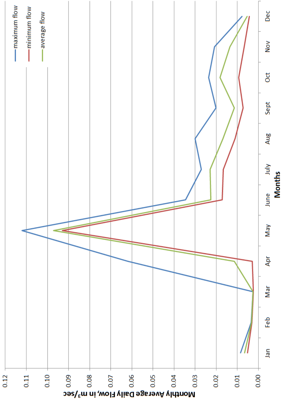
Figure 17E.23 Maximum, Minimum, and Average Flow Hydrographs of Subwatershed #21
