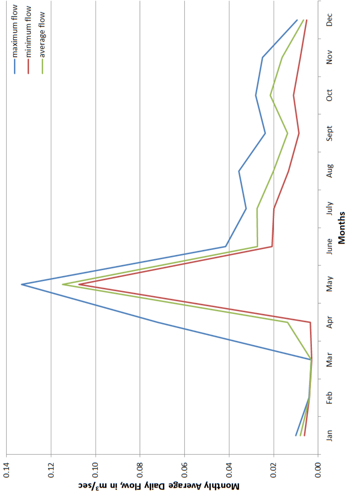
Figure 17E.5 Maximum, Minimum, and Average Flow Hydrographs of Subwatershed #4
