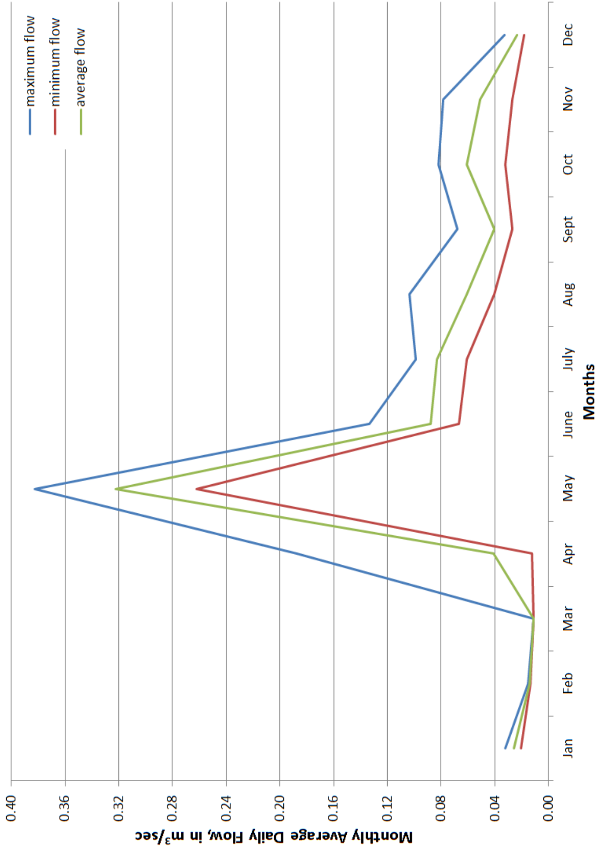
Figure 17E.11 Maximum, Minimum, and Average Flow Hydrographs of Subwatershed #10
