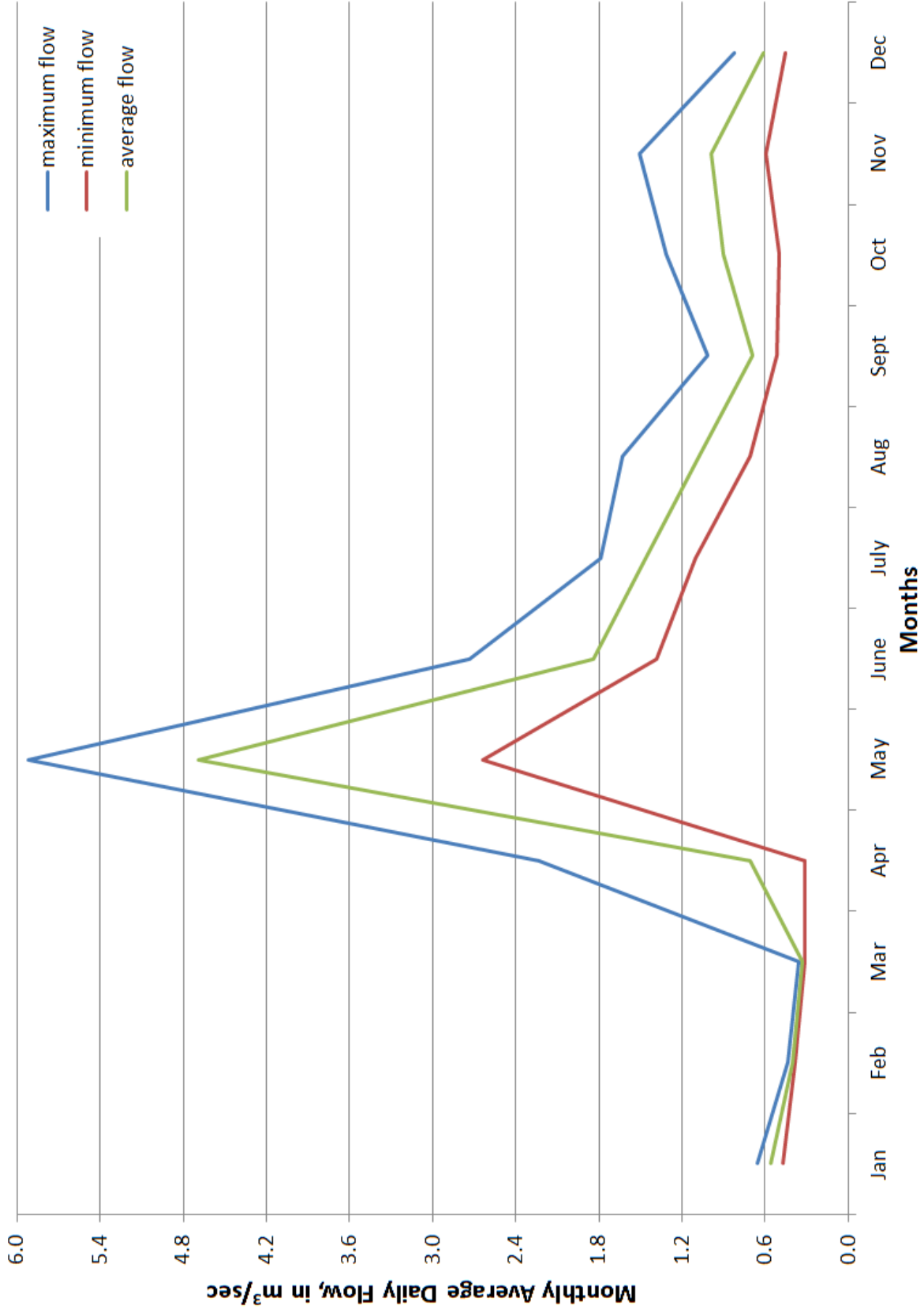
Figure 17E.14 Maximum, Minimum, and Average Flow Hydrographs of Subwatershed #13
