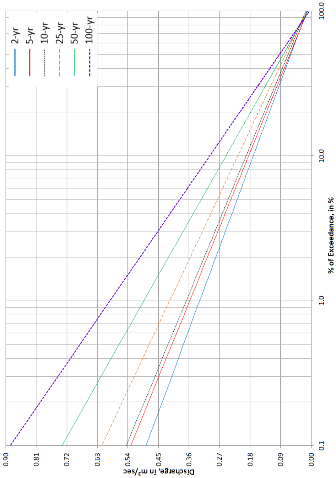
Figure 17F.16 Flow Duration Curves of Subwatershed #15
