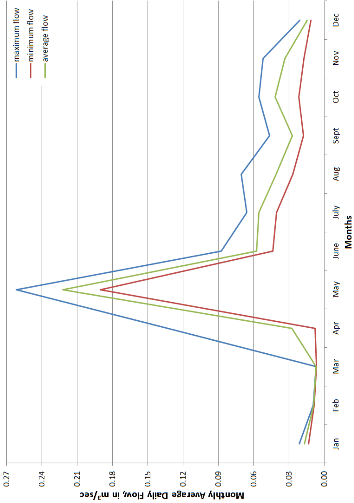
Figure 17E.13 Maximum, Minimum, and Average Flow Hydrographs of Subwatershed #12
