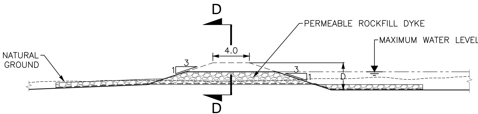
TYPICAL SECTION PERMEABLE ROCKFILL DYKE AND EMERGENCY SPILLWAY
