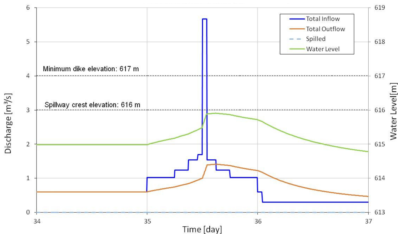
Figure 7-4: 25 Years Flood Routing through Sedimentation Pond HOWSEB
