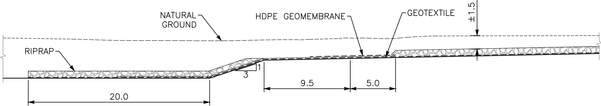
SECTION C-C
