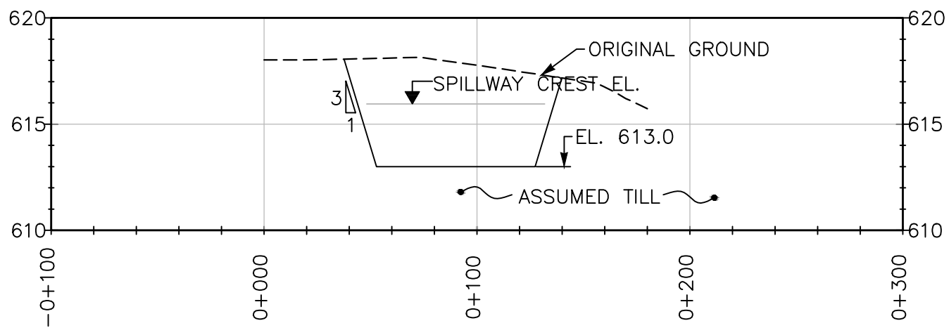
SECTION B-B - SEDIMENTATION POND HOWSE B
