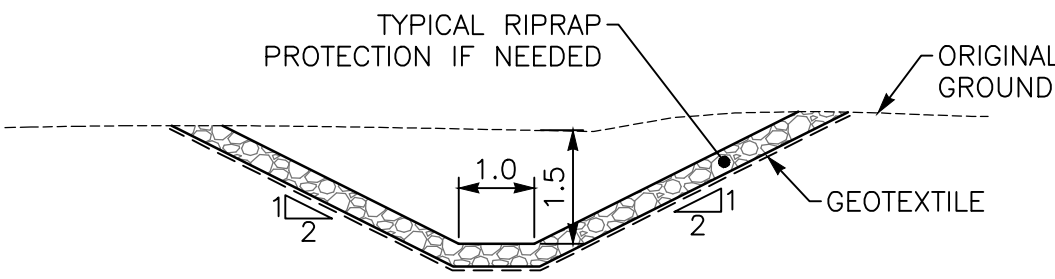
TYPICAL DITCH SECTION (NOTE 2)
