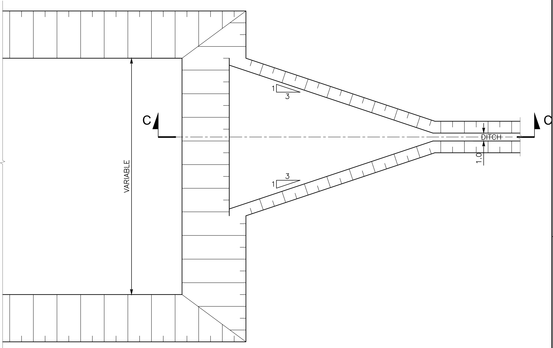
TYPICAL POND ENTRANCE DETAIL
