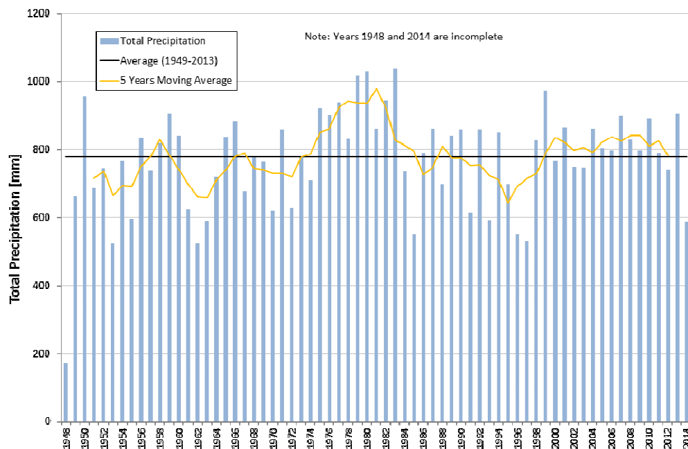
Figure 2-1: Total Precipitation (1948-2014)
