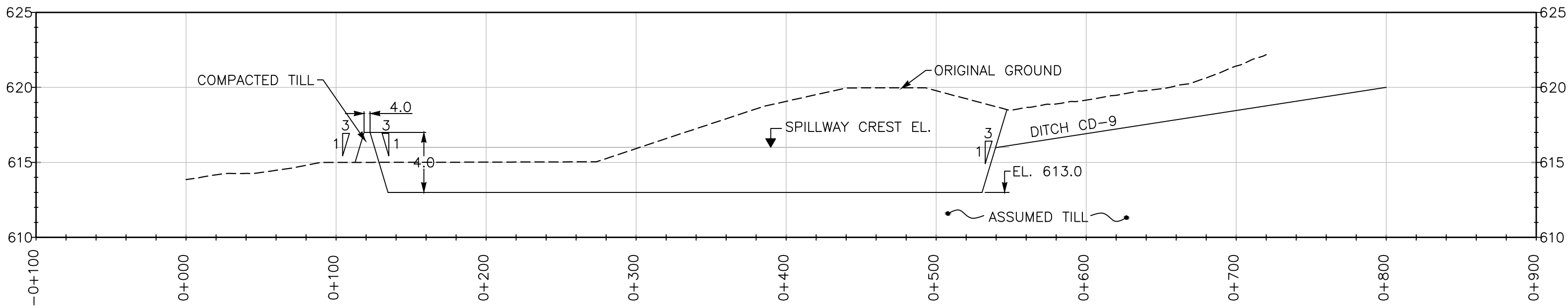
SECTION A-A - SEDIMENTATION POND HOWSE B
