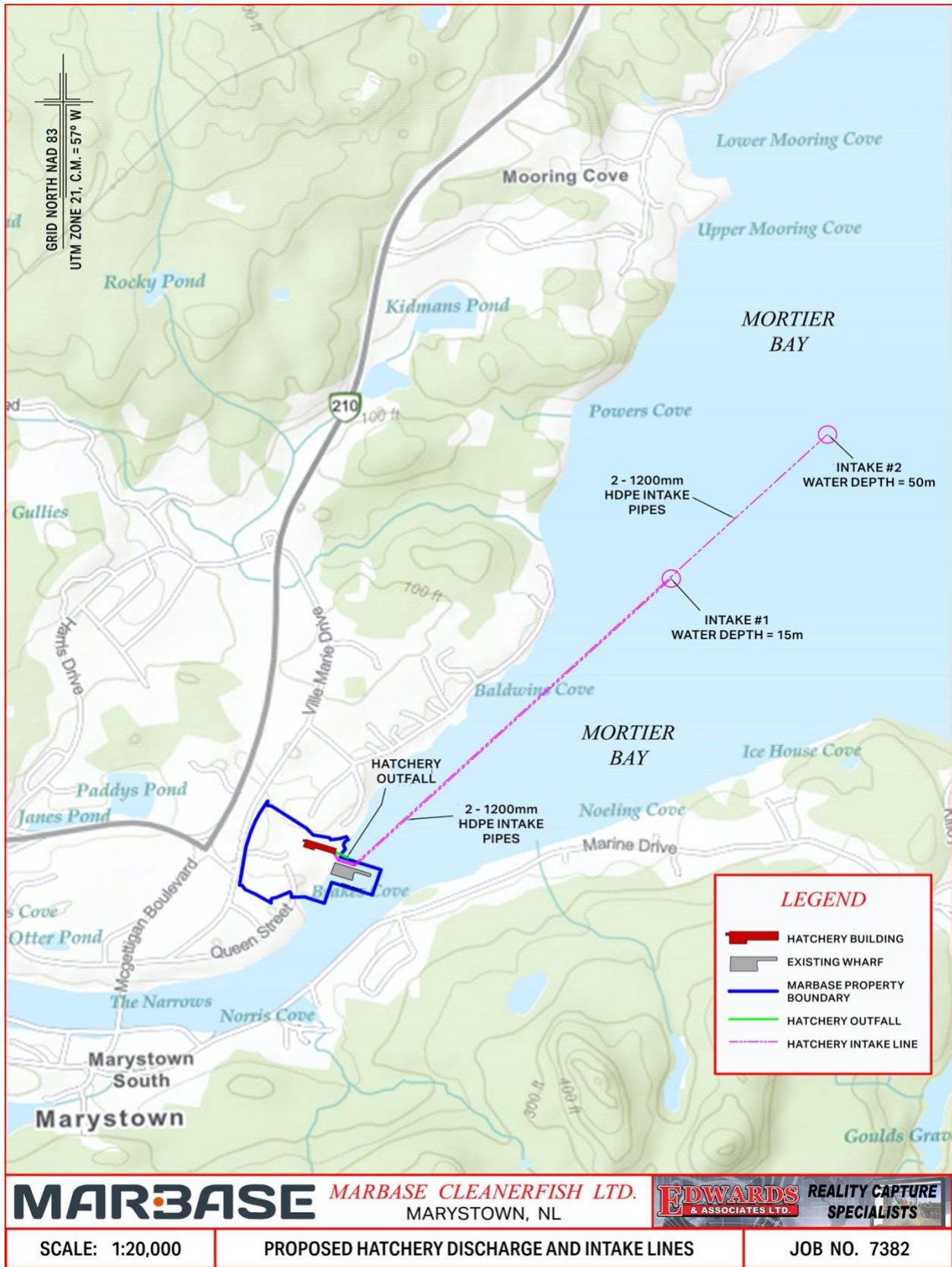
Figure 4.4: Proposed Marbase Hatchery Sea Water Supply
