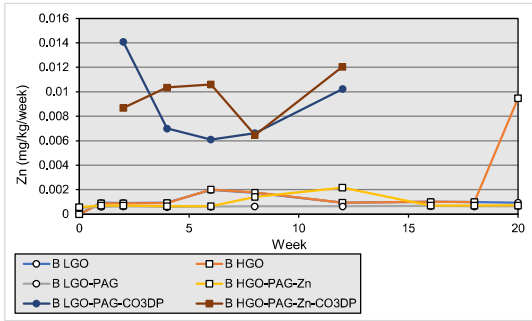
Figure C-2: Berry Ore and Overburden Humidity Cell Plots
