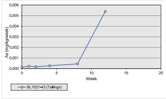
Figure C-3: Berry Tailings Subaqueous Cell Plots
