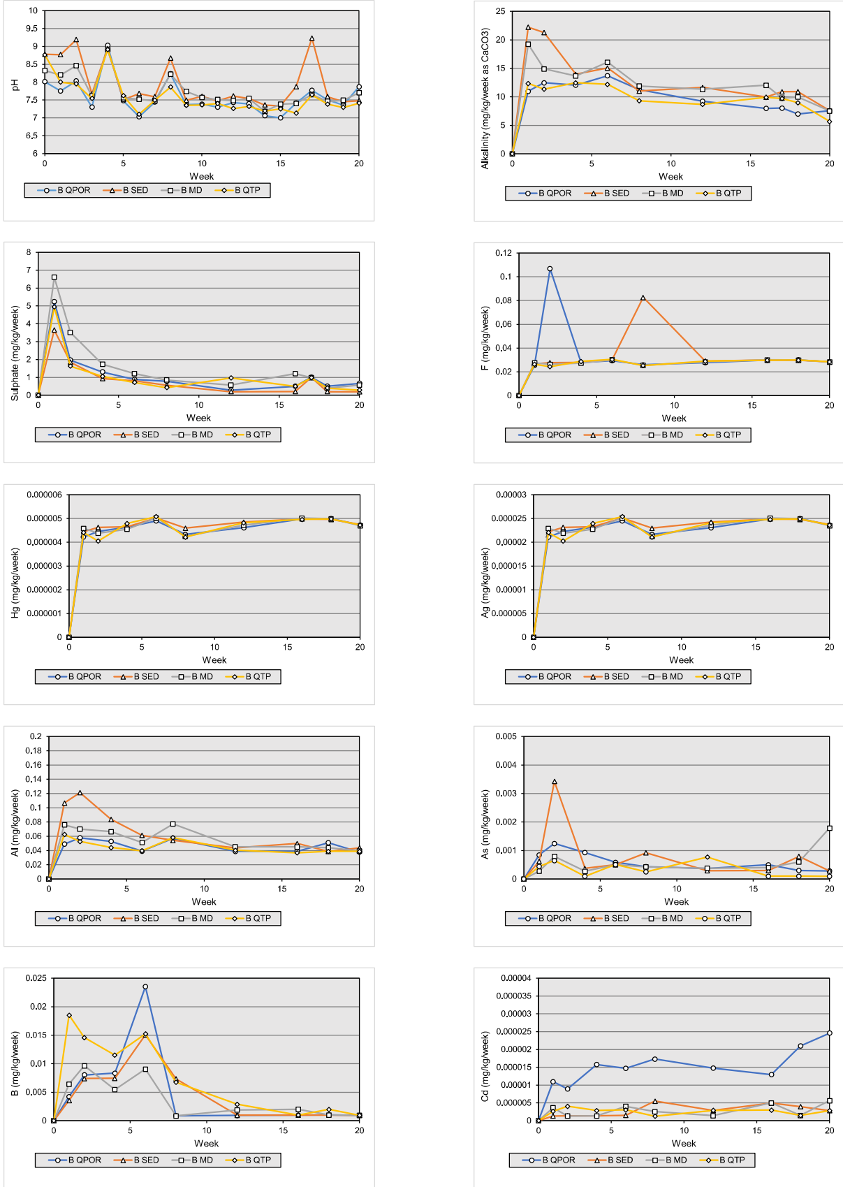
Figure C-1: Berry Waste Rock Humidity Cell Plots
