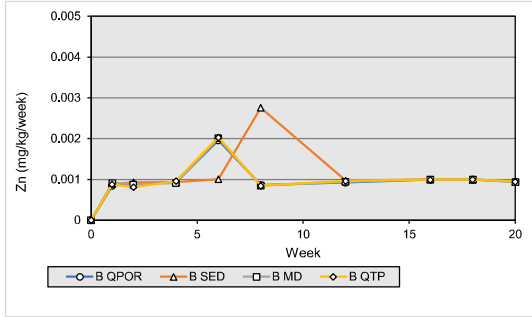
Figure C-1: Berry Waste Rock Humidity Cell Plots
