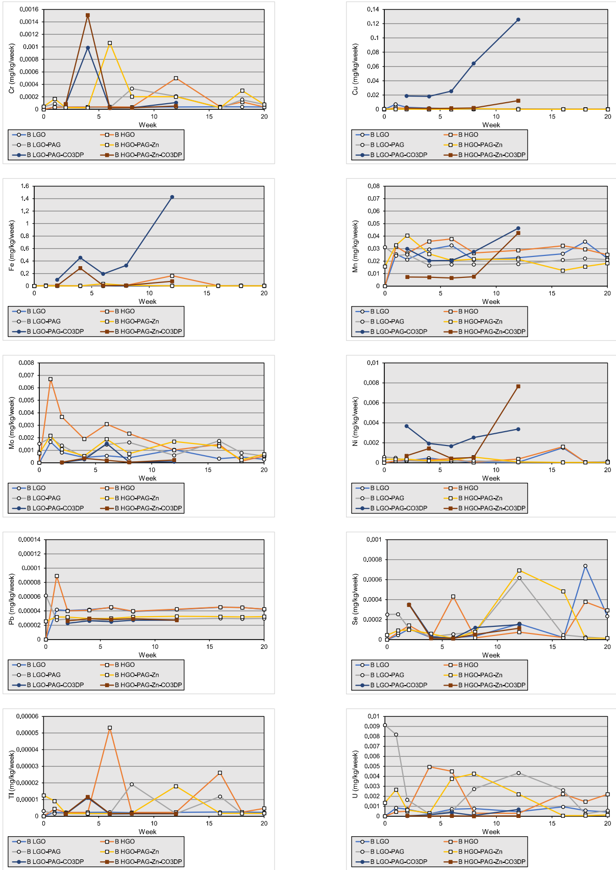
Figure C-2: Berry Ore and Overburden Humidity Cell Plots
