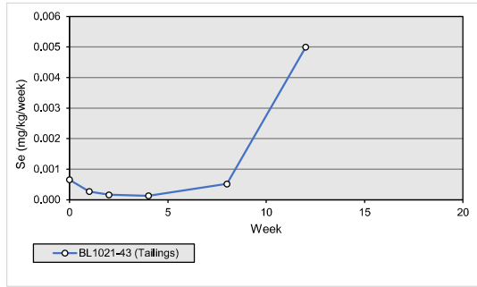
Figure C-3: Berry Tailings Subaqueous Cell Plots
