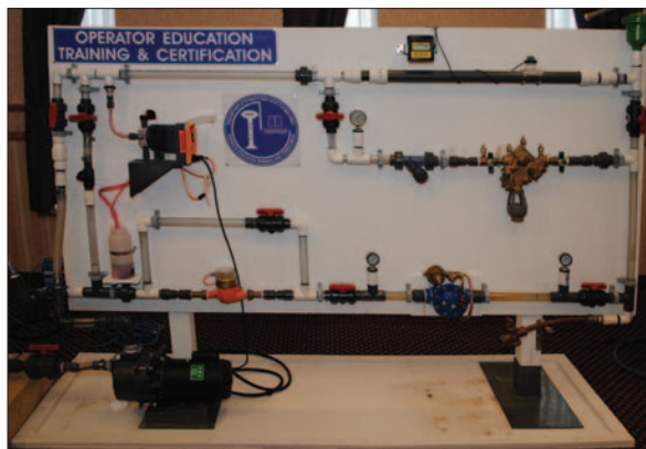
Water distribution system working model
