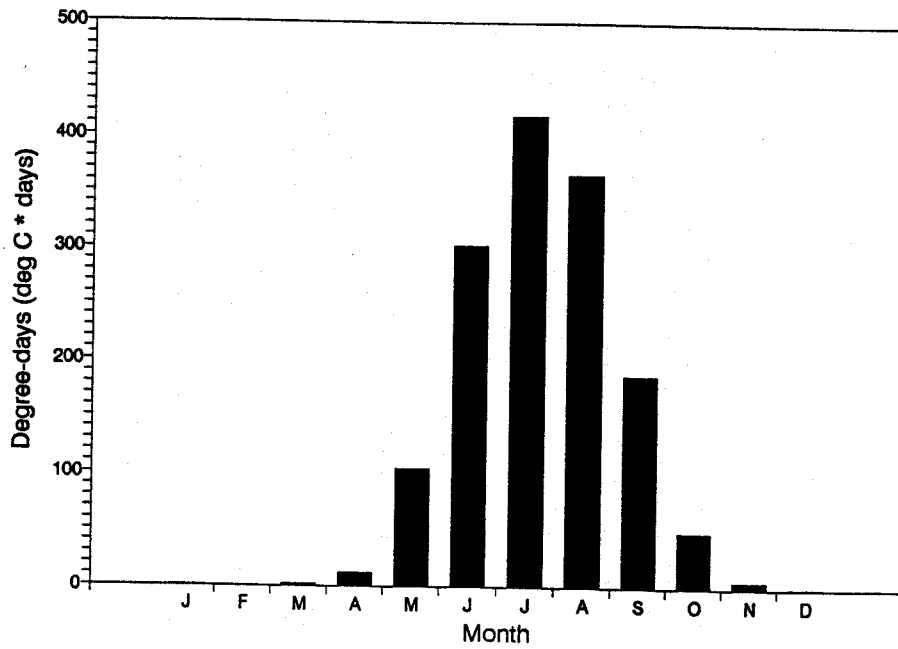
Mean Monthly Melting Degree-days (1951-80 normals) WABUSH LAKE A
