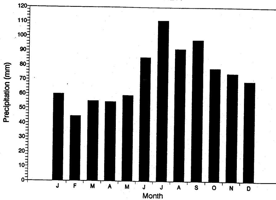
Mean Monthly Precipitation (1961-90 normals) WABUSH LAKE A
