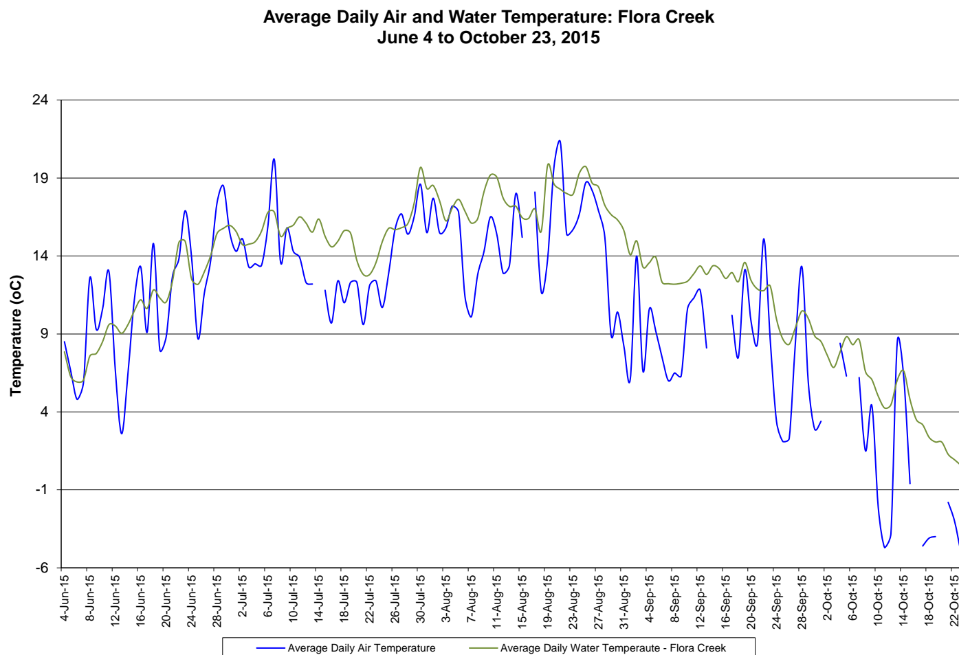
Figure 2: Average daily air and water temperatures – Flora Creek below TLH (Weather data collected at Churchill Falls)
