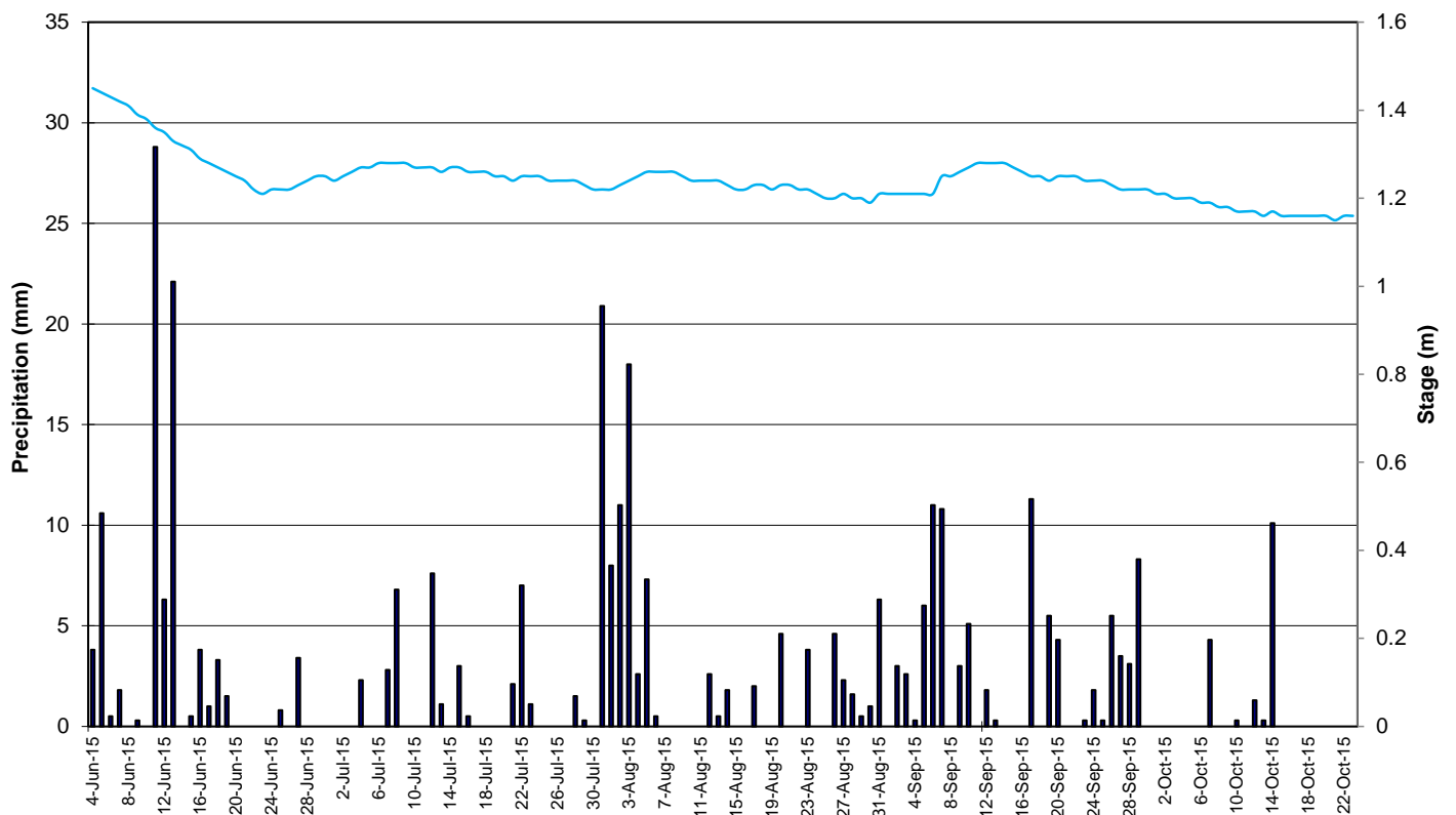
Figure 7: Stage and precipitation at Flora Creek below TLH (Weather data collected at Churchill Falls)
