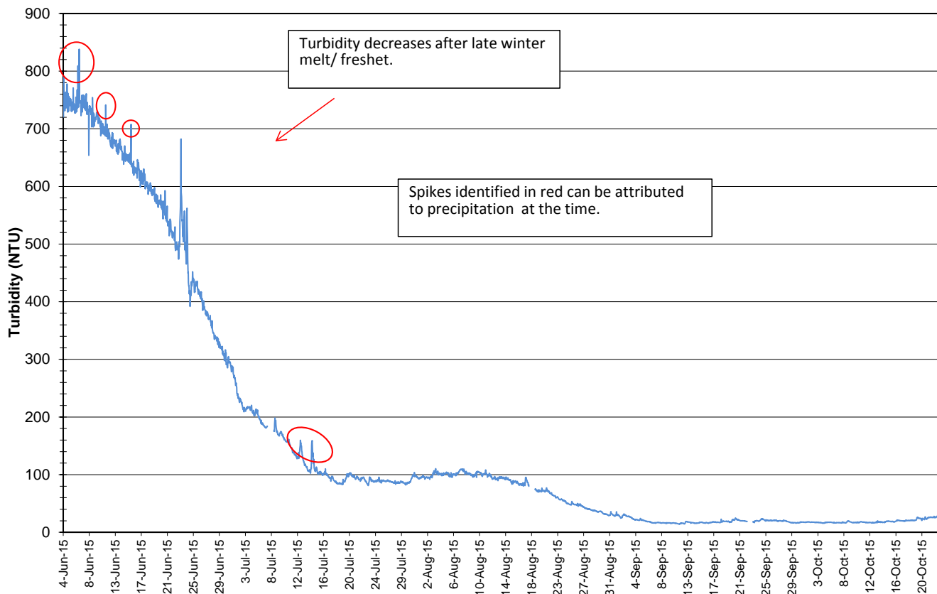
Water Turbidity: Flora Creek below TLH June 4 - October 23, 2015
