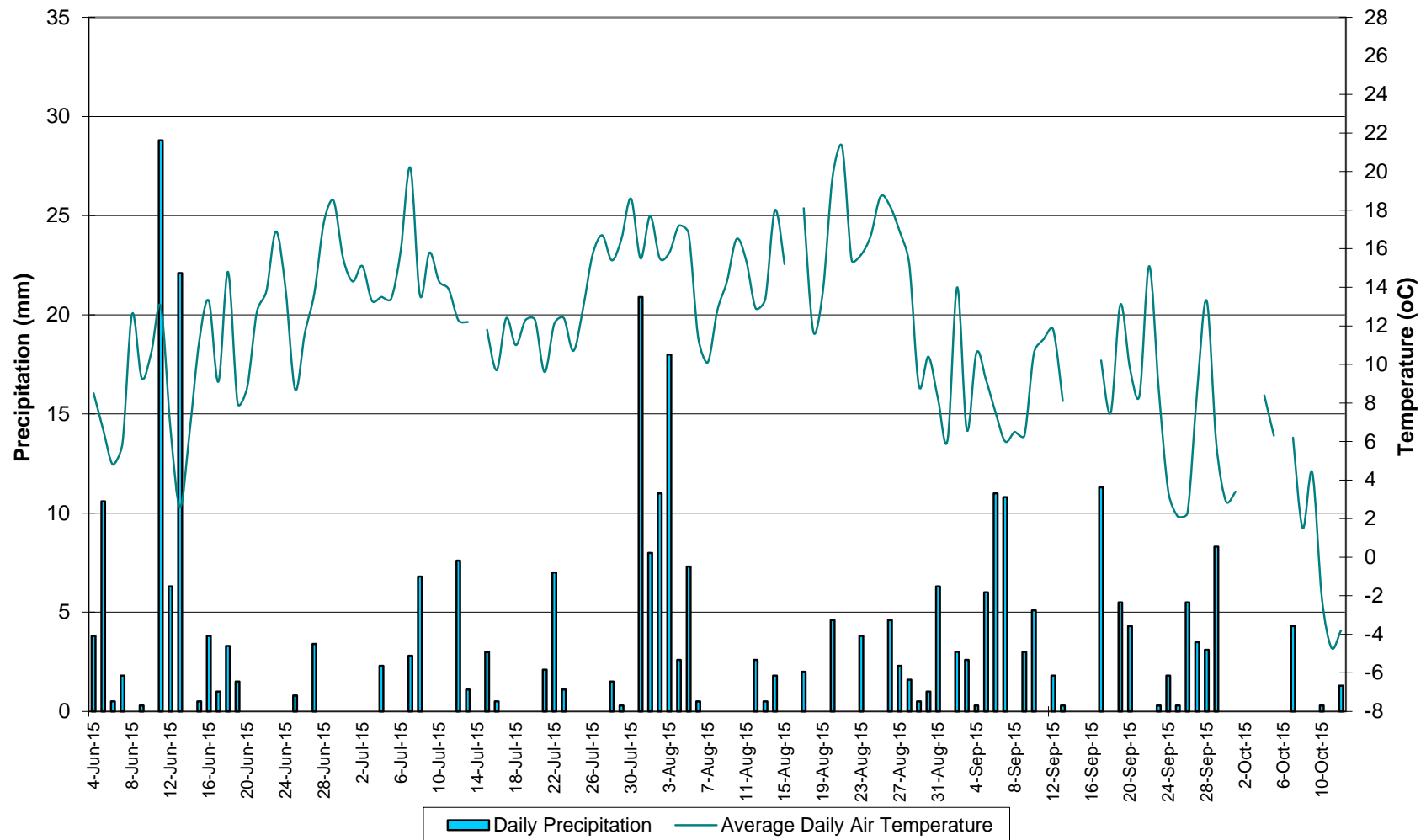
Average Daily Air Temperature and Daily Precipitation: Churchill Falls, NL June 4 to October 23, 2015
