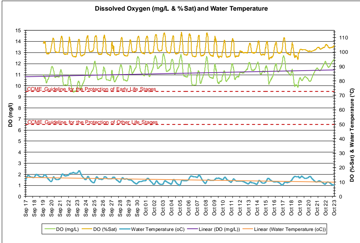
Figure 4: Dissolved Oxygen (concentration and percent saturation) at Waterford River at Kilbride Station
