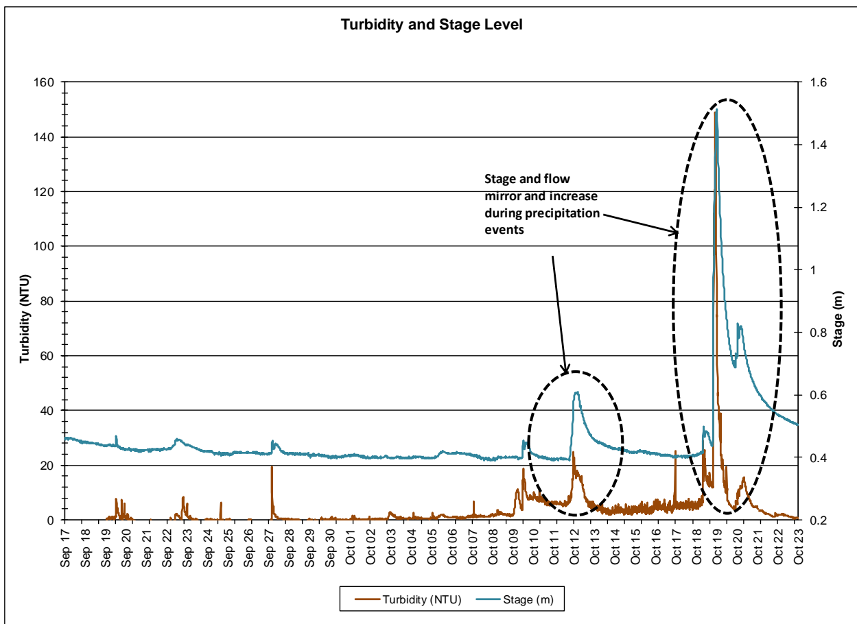
Figure 5: Turbidity (NTU) and Stage Level (m) at Waterford River at Kilbride Station
