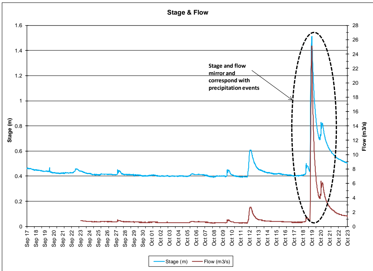
Figure 7: Stage and Flow at Waterford River at Kilbride Station
