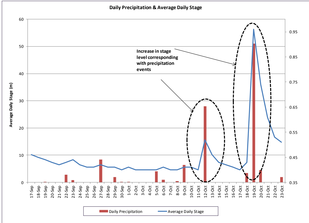
Figure 6: Average daily stage (m) at Waterford River at Kilbride Station and Daily Precipitation (mm) at St. John's International Airport
