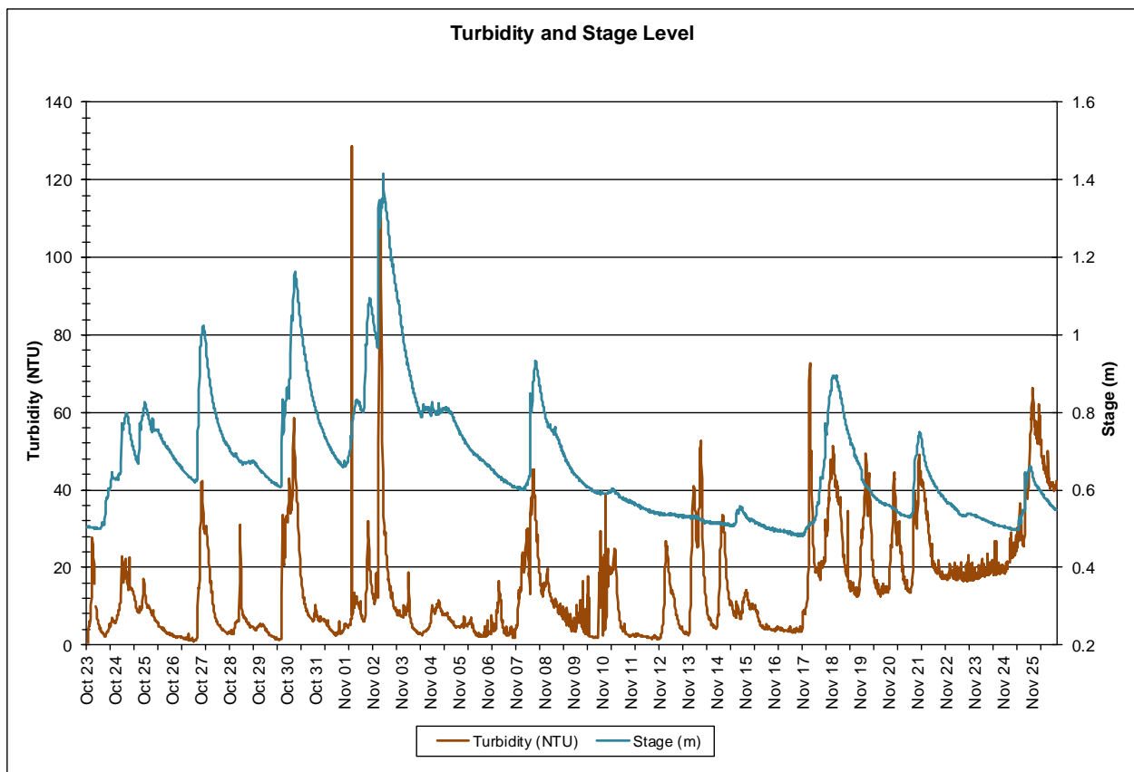
Figure 5: Turbidity (NTU) and Stage Level (m) at Waterford River at Kilbride Station
