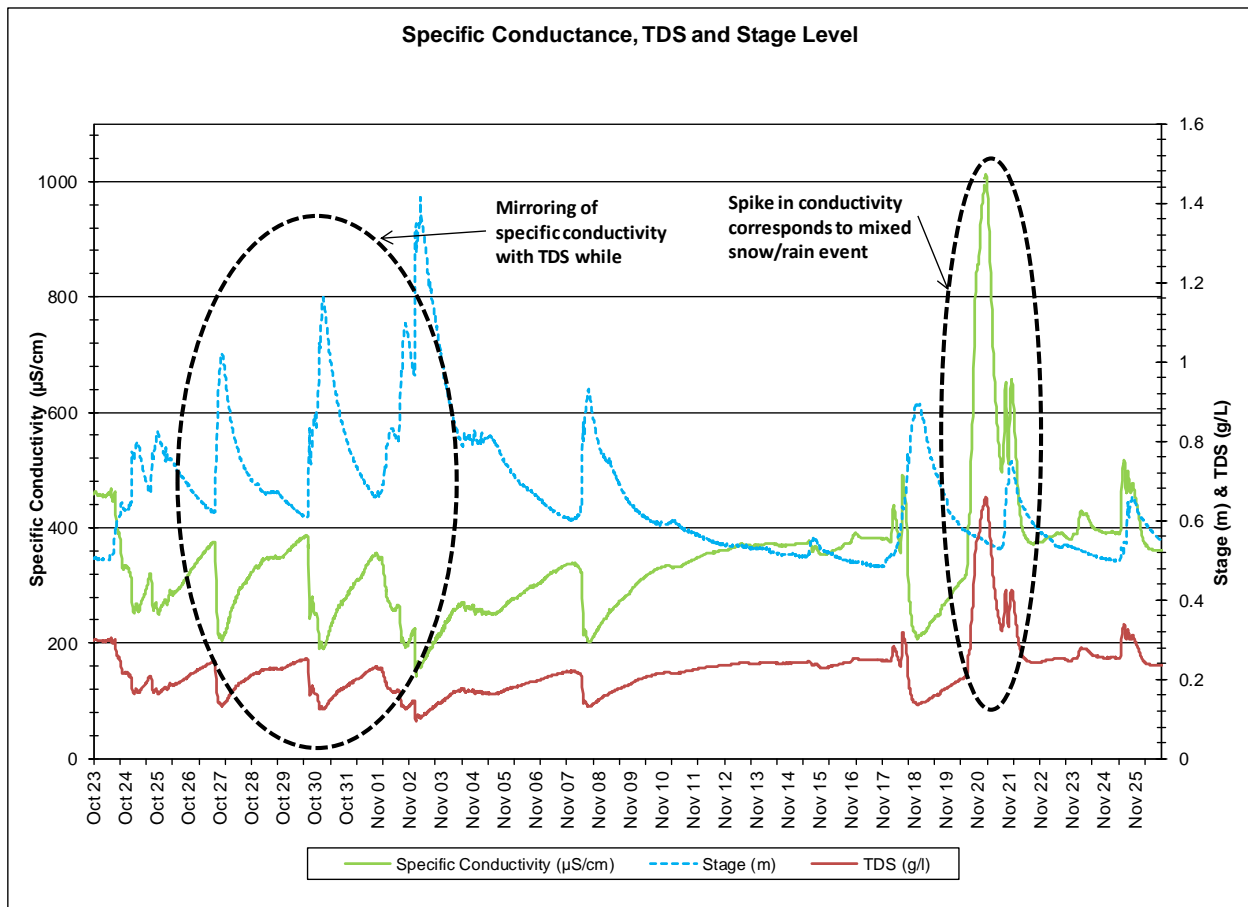
Figure 3: Specific conductivity (uS/cm), TDS (g/L) and stage (m) values for Waterford River at Kilbride Station
