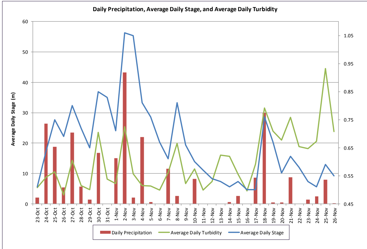
Figure 6: Average daily turbidity (NTU), and Average daily stage (m) at Waterford River at Kilbride Station and Daily Precipitation (mm) at St. John's International Airport
